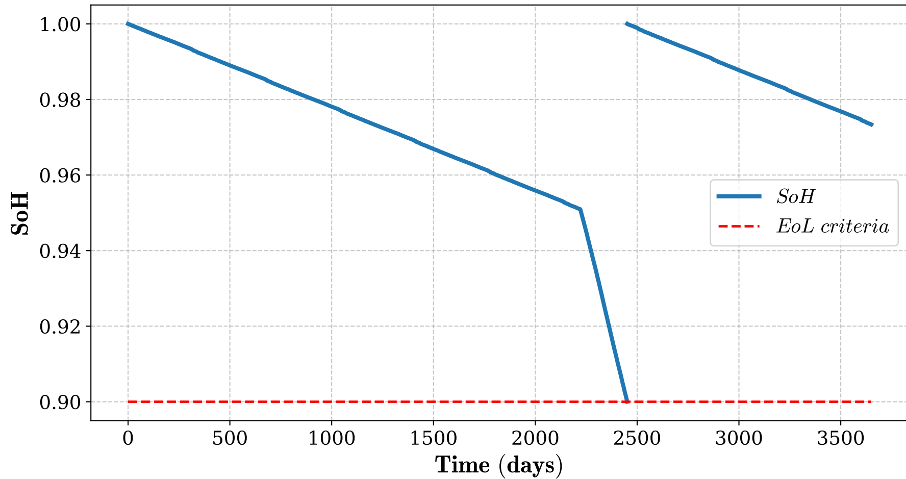
SoH of the fuel cell
