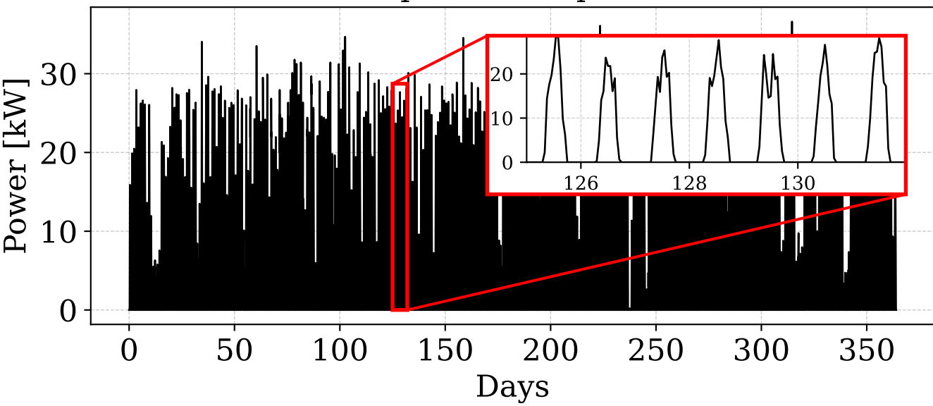
PV production profile
