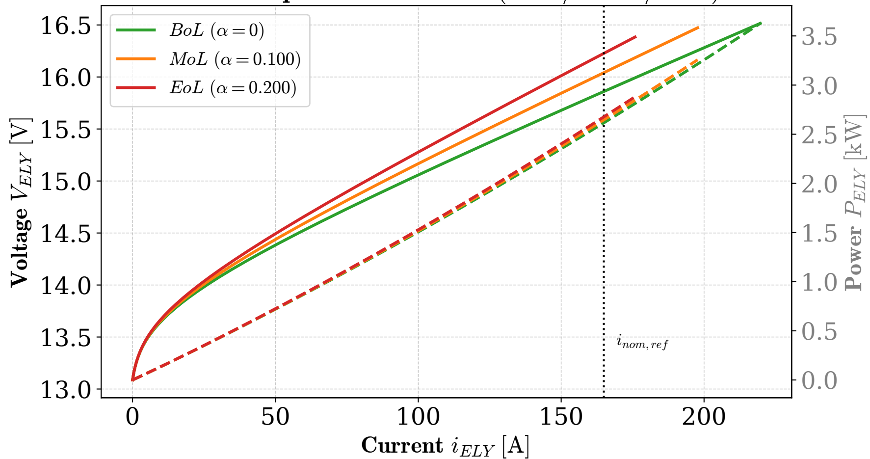
PEMWE polarization curve (BoL / MoL / EoL)
