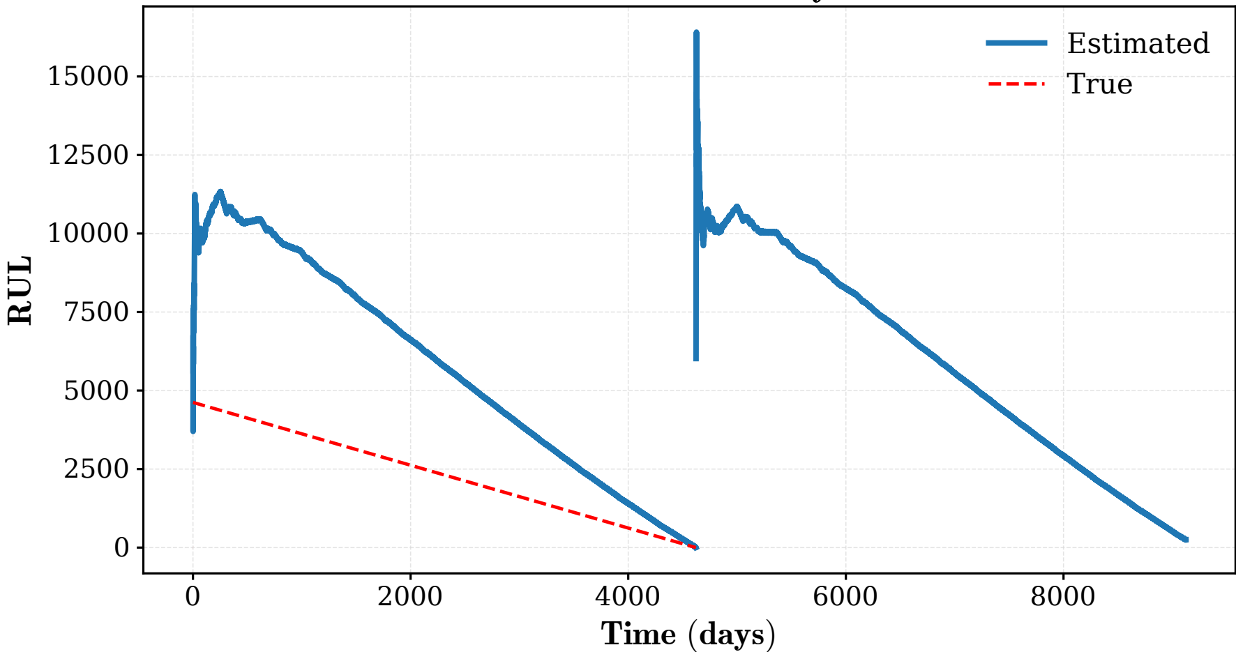
RUL of the electrolyzer
