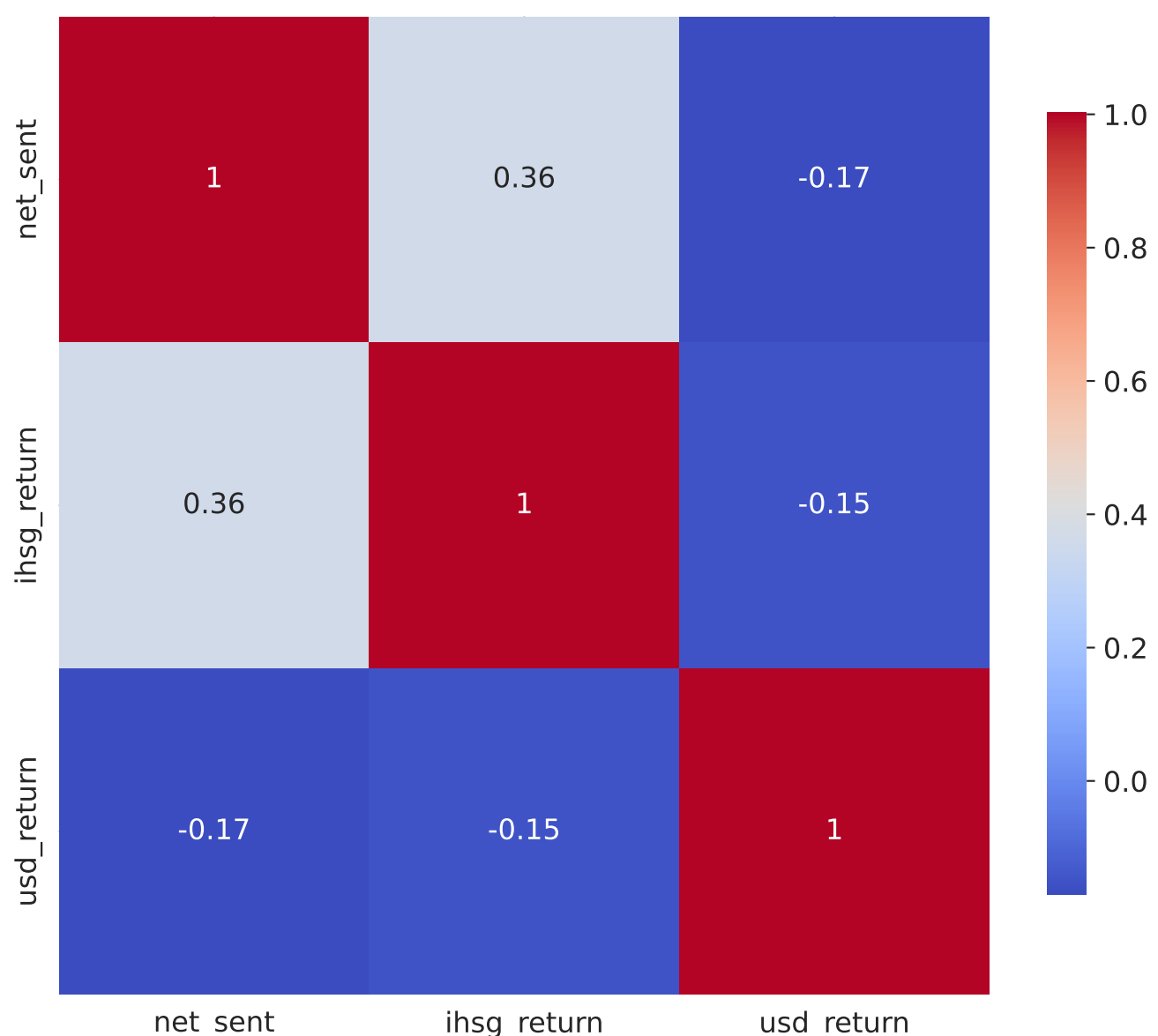
Correlation Heatmap
