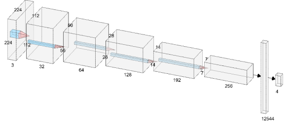
Fig. 2: CNN Architecture
