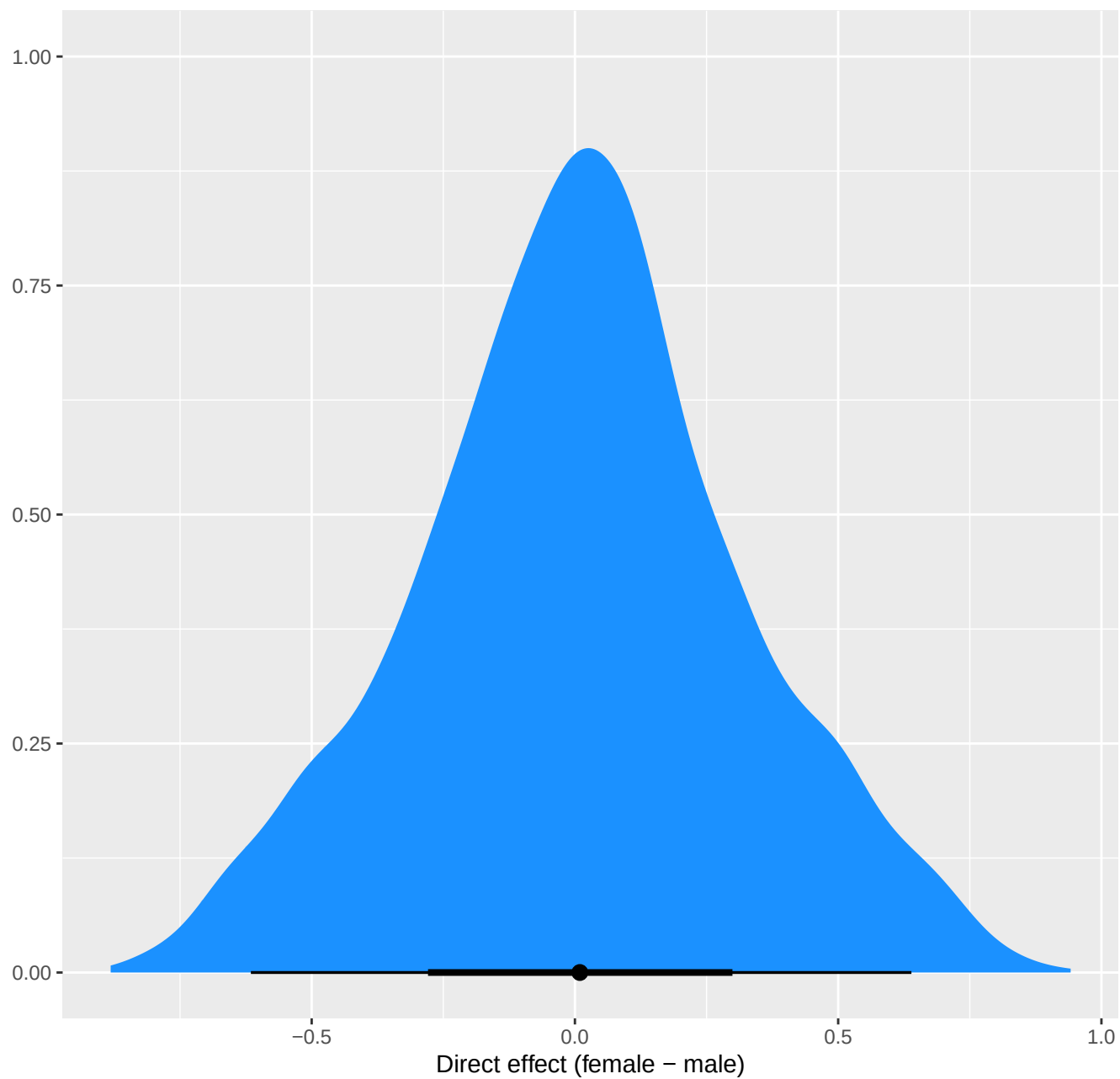
Prior on the estimand
