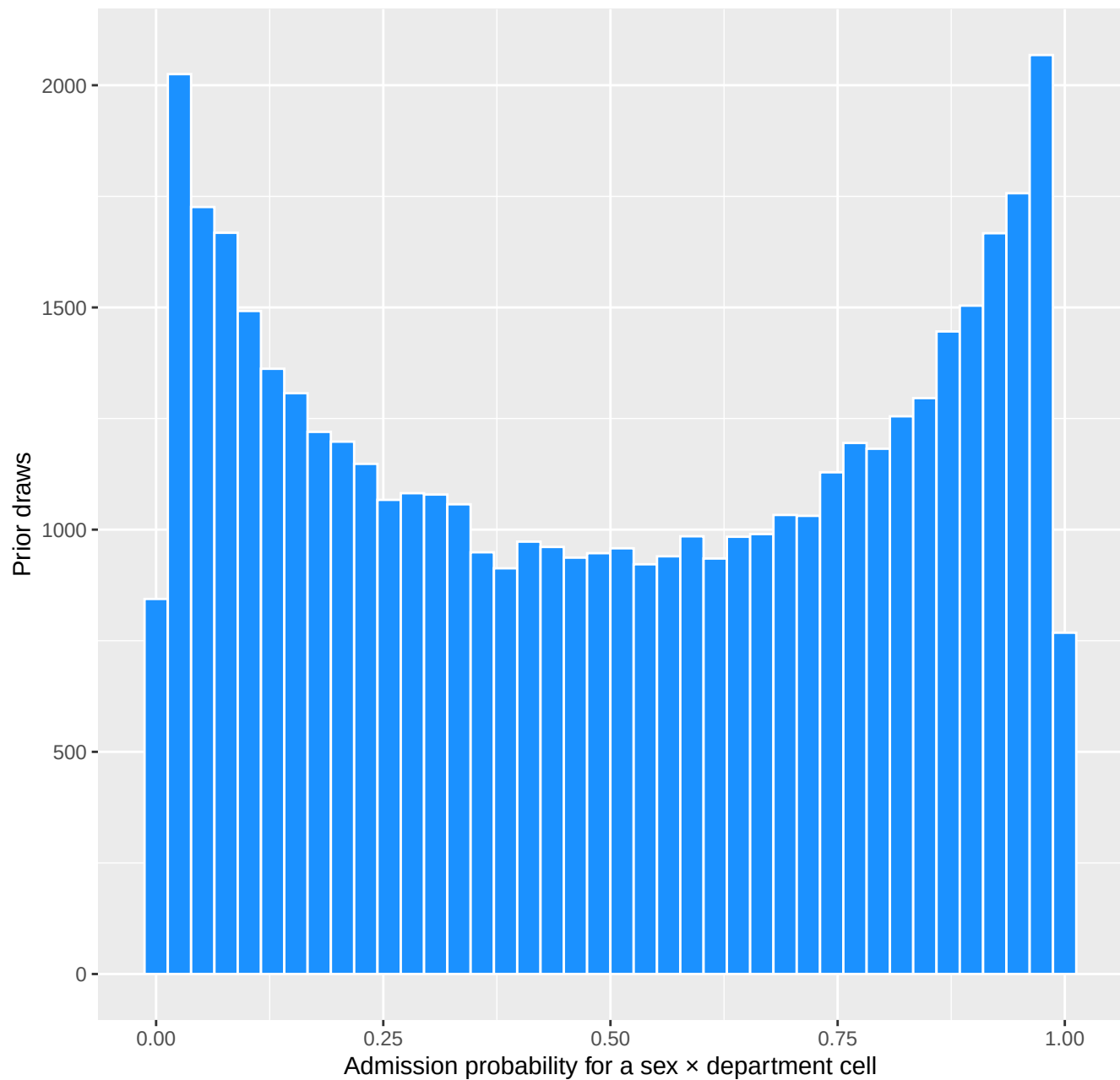
What the priors imply about admission rates
