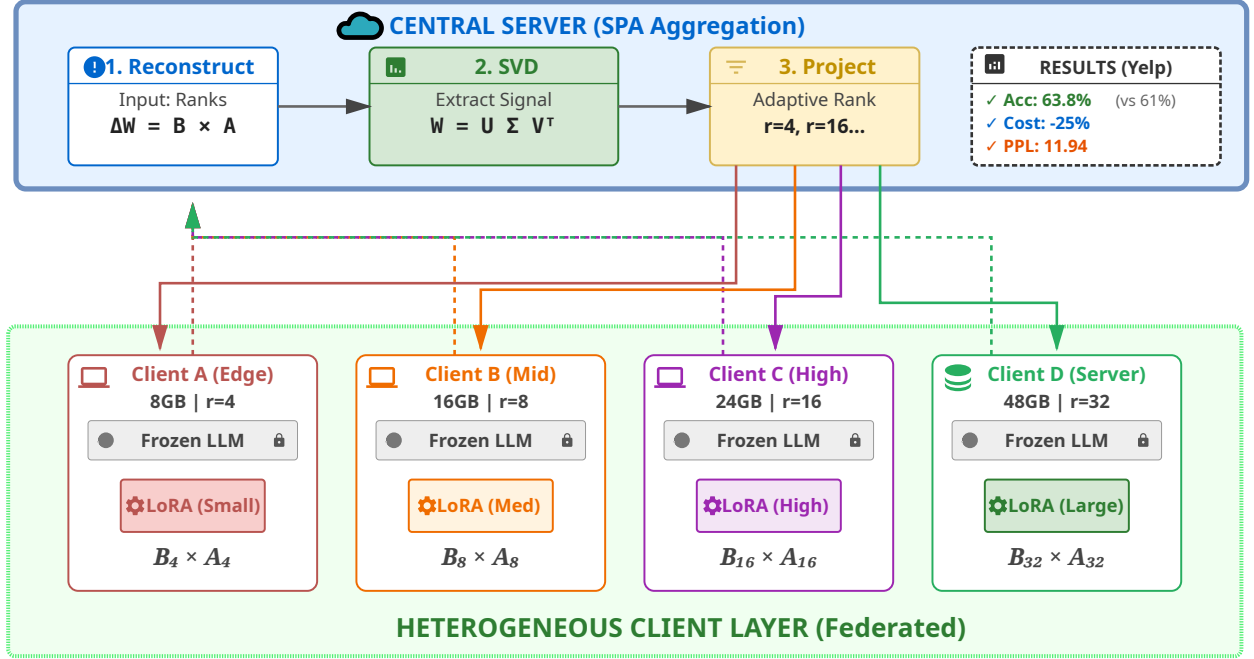
Fig. 2: System Architecture of Heterogeneous Decentralized Fine-Tuning with Subspace Projection Aggregation (SPA).
