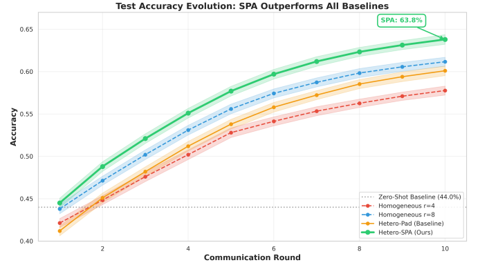
Fig. 5: Test accuracy evolution across communication rounds. The dashed horizontal line at 44% represents the zero-shot baseline (pre-trained model without fine-tuning). SPA consistently outperforms all baselines, achieving 63.8\% \pm 0.7\% final accuracy compared to 61.2\% \pm 0.7\% for Homogeneous r=8 .
