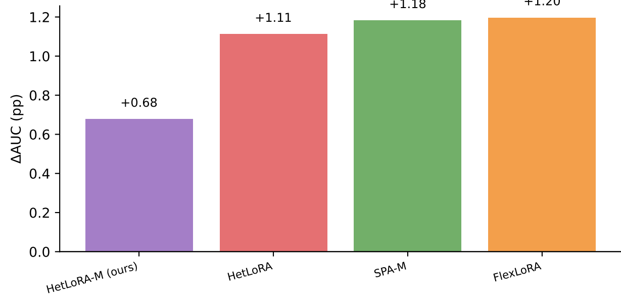
\Delta AUC (skewed – balanced)
