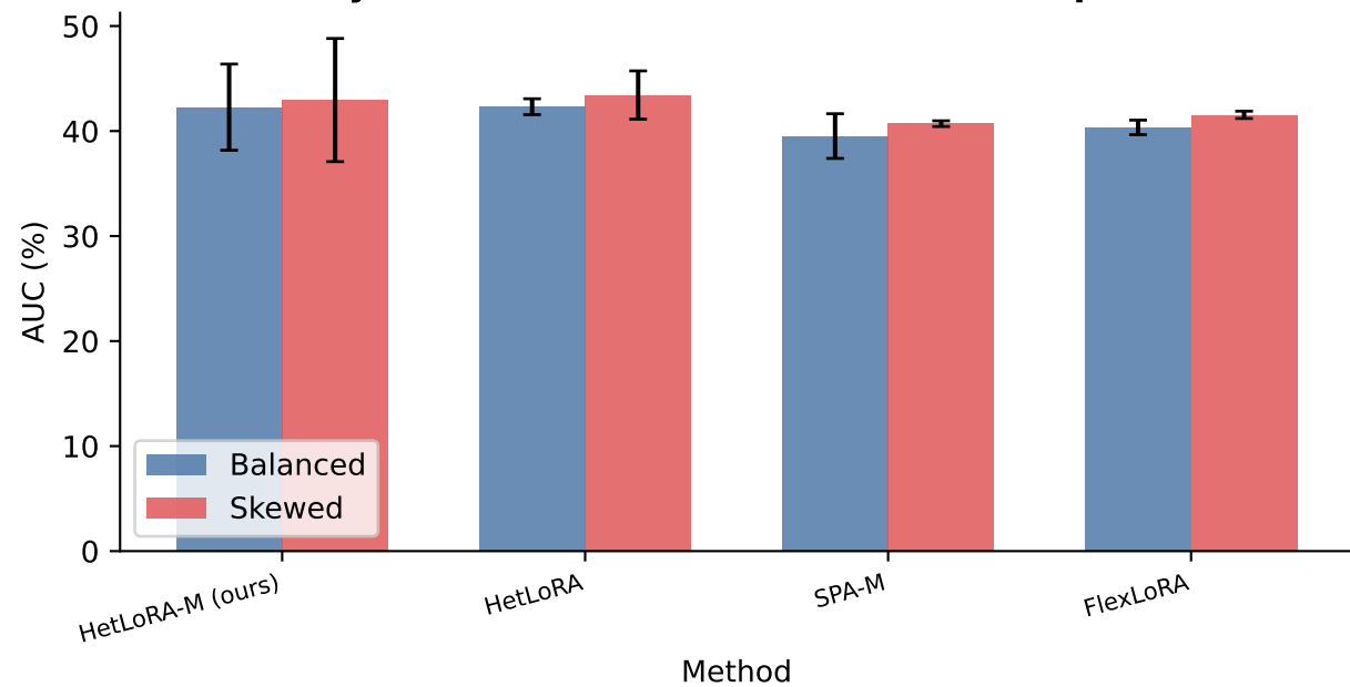
AUC by Method and Rank Distribution (Yelp \alpha=0.1 )
