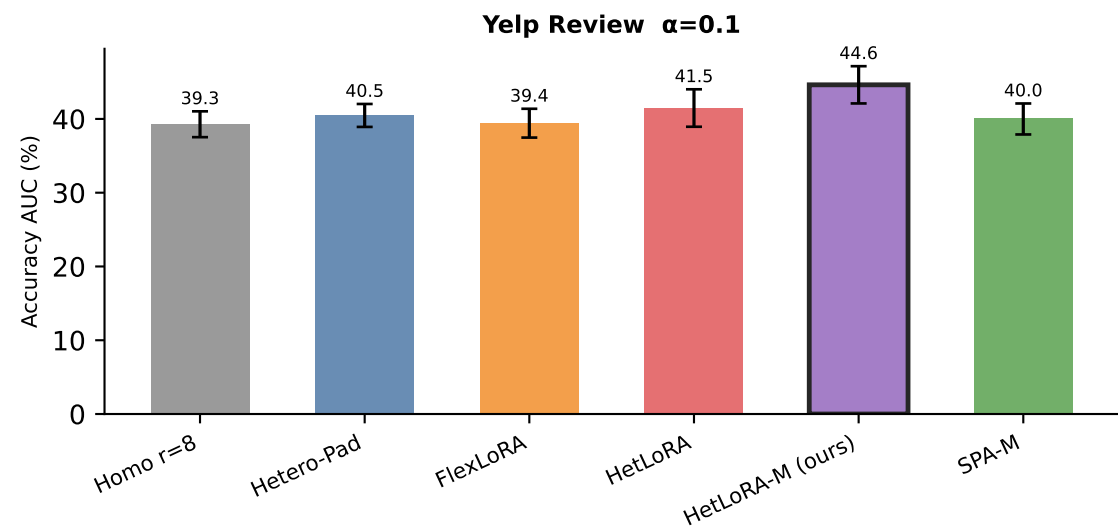
AUC (mean across all rounds) \pm std
