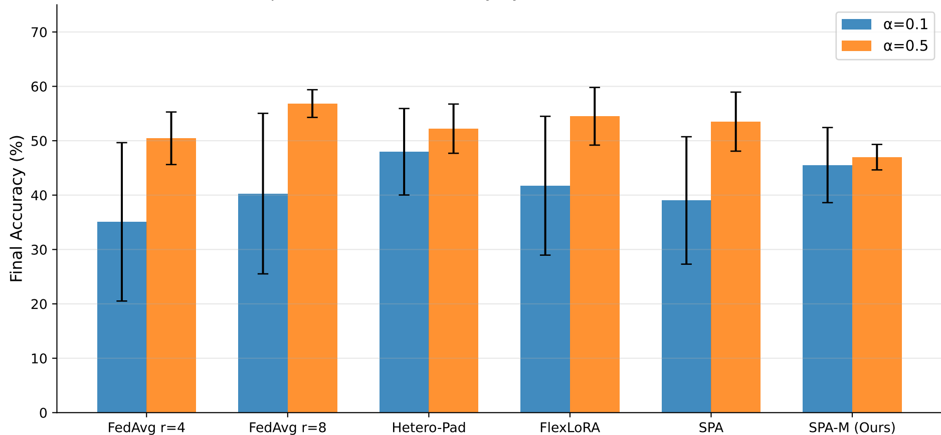
Yelp — Final Round Accuracy by Method and Non-IID Level
