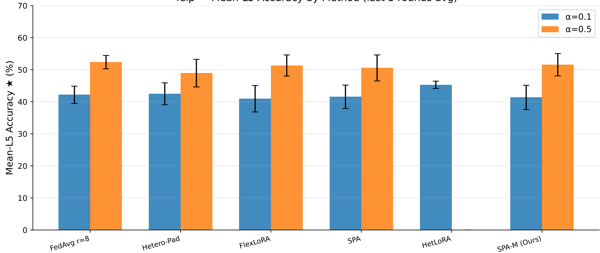
Yelp — Mean-L5 Accuracy by Method (last 5 rounds avg)
