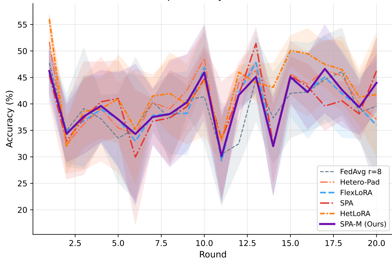
Yelp Accuracy — \alpha=0.1
