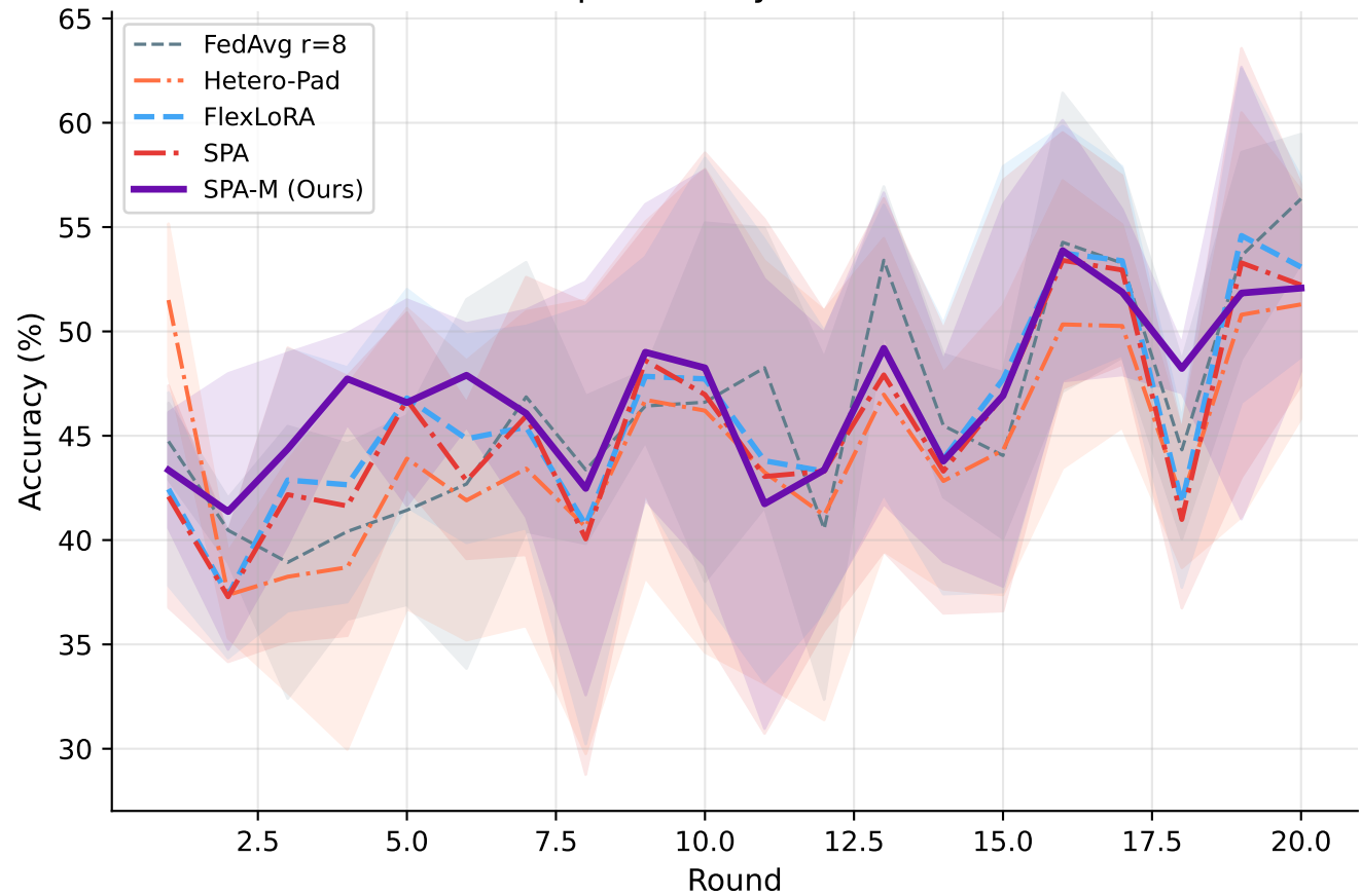
Yelp Accuracy — \alpha=0.5
