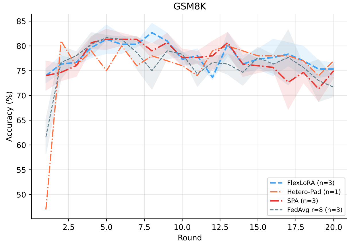
Cross-Dataset Accuracy ( \alpha=0.5 , mean \pm std)
