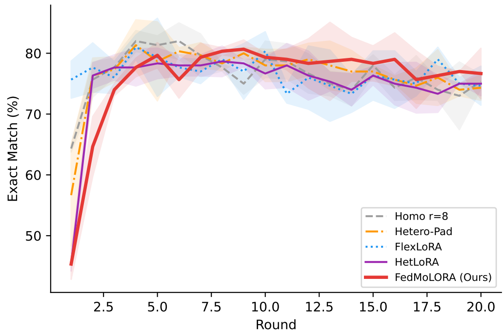
GSM8K \alpha=0.1
