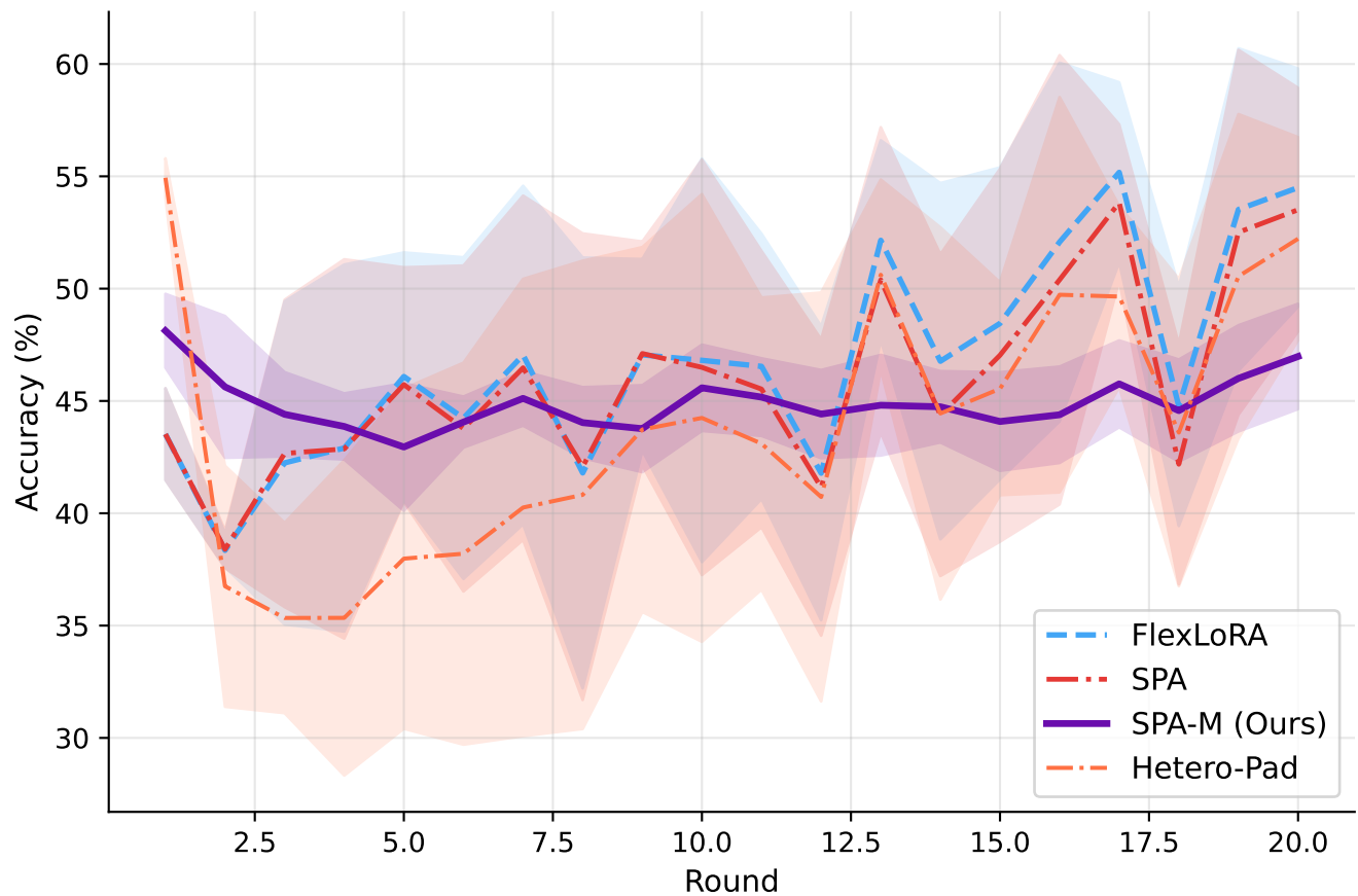
SPA-M vs SPA vs FlexLoRA — \alpha=0.5
