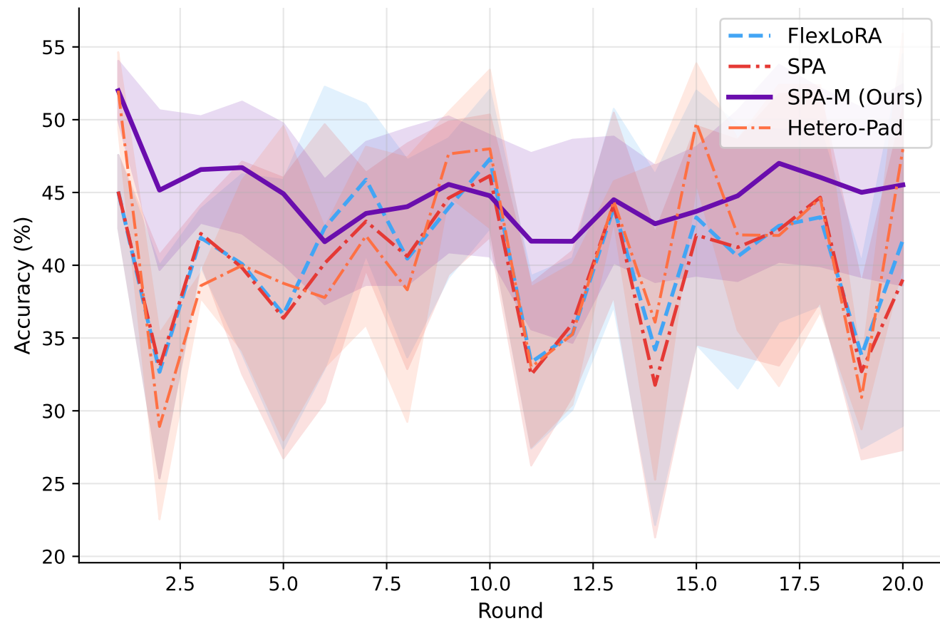
SPA-M vs SPA vs FlexLoRA — \alpha=0.1
