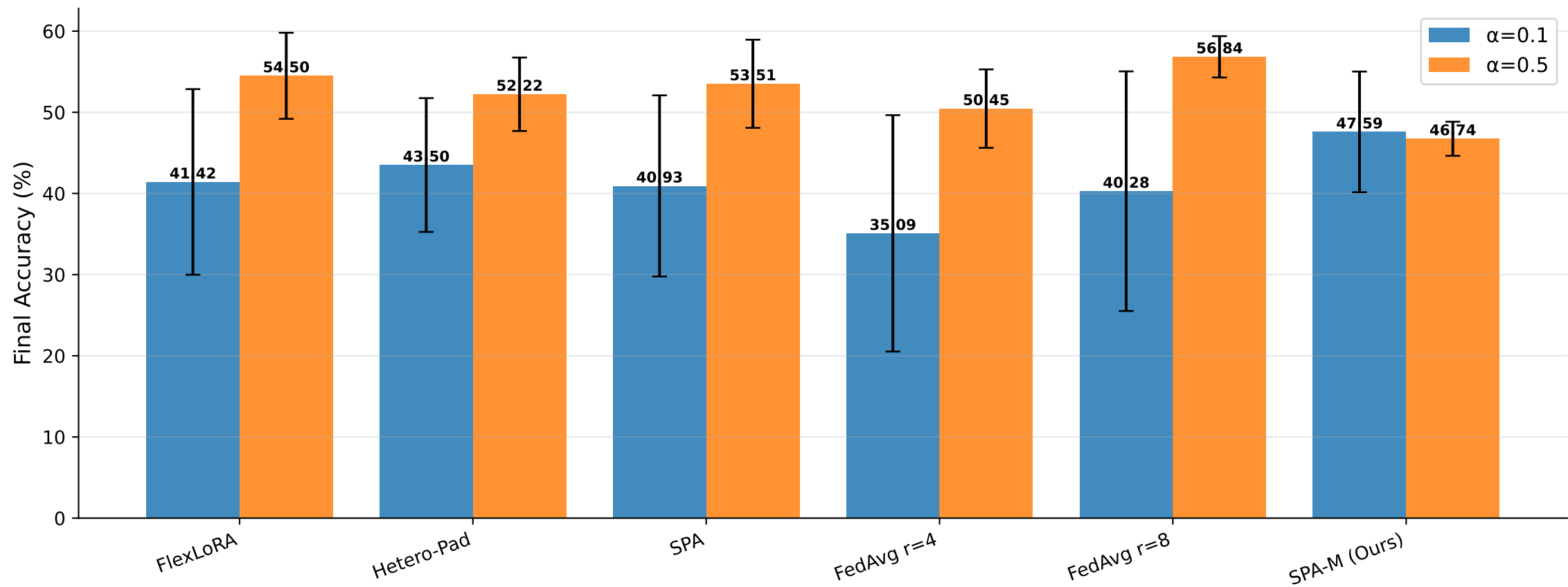
YELP — Final Accuracy (%) by Method & \alpha
