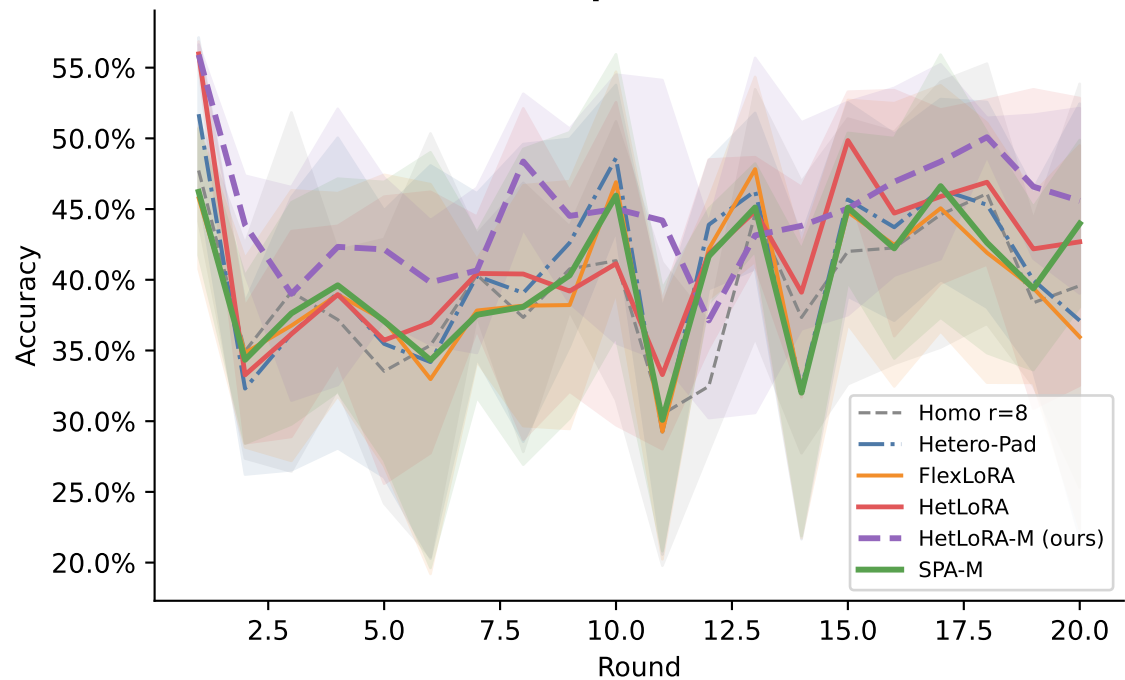
Yelp \alpha=0.1
