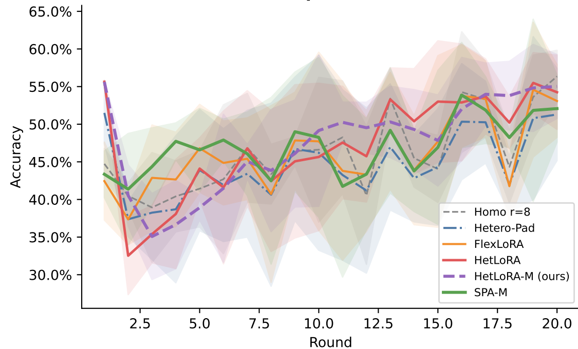
Yelp \alpha=0.5
