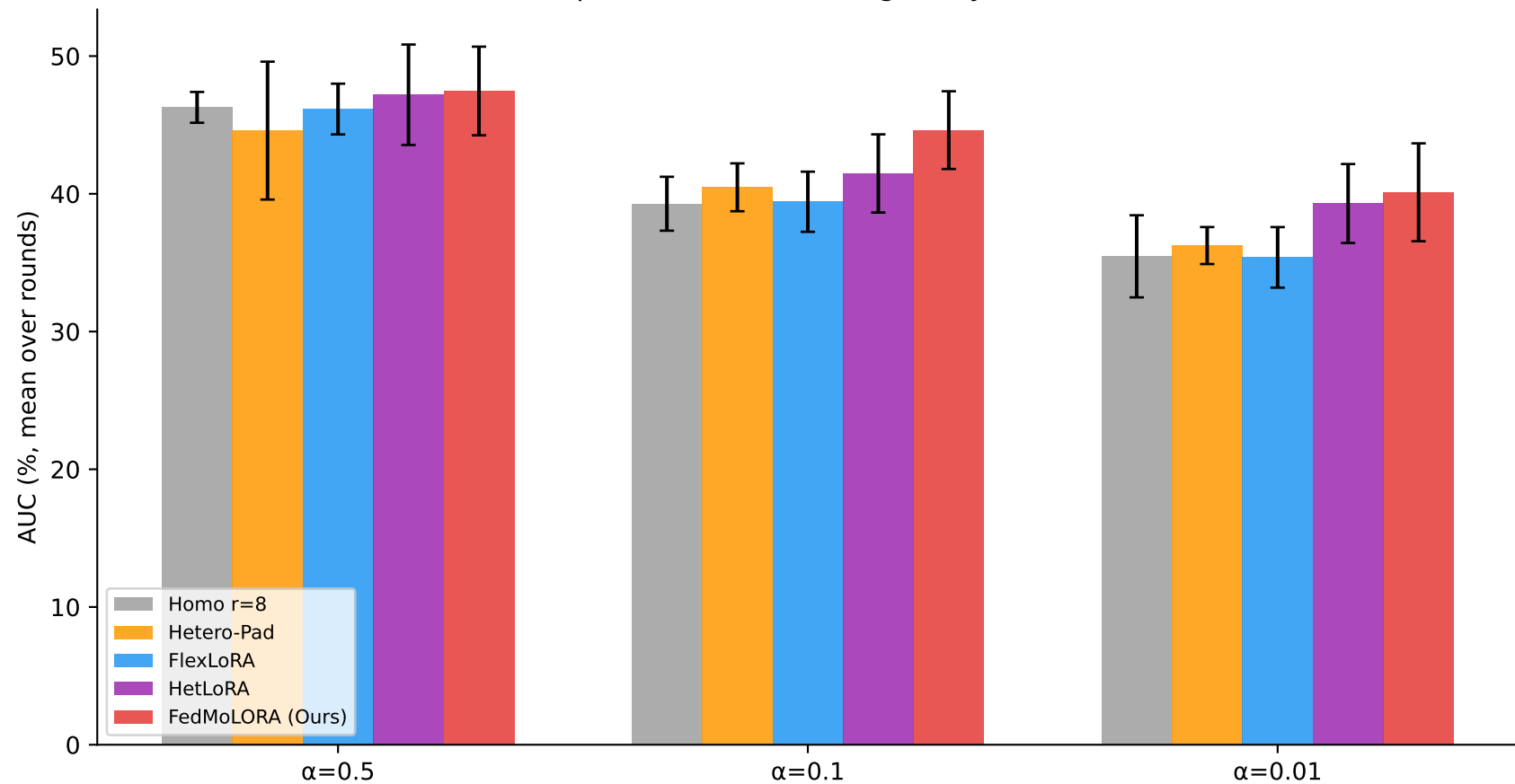
Yelp: AUC across heterogeneity levels
