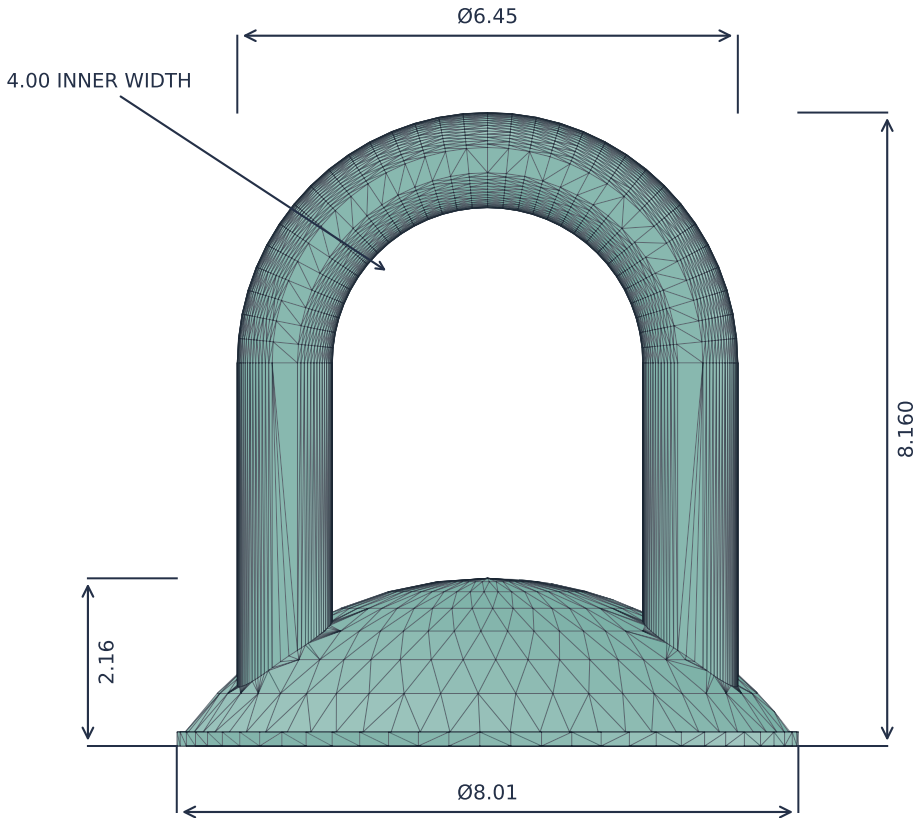
FRONT VIEW - DIMENSIONED
