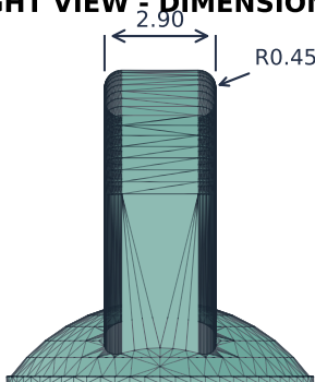
RIGHT VIEW - DIMENSIONED
