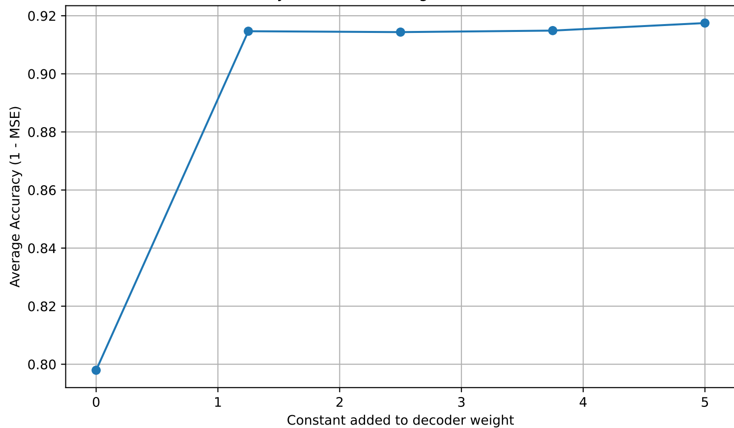
FM Accuracy vs. Decoder Weight Constant ( \epsilon = 0.001 )
