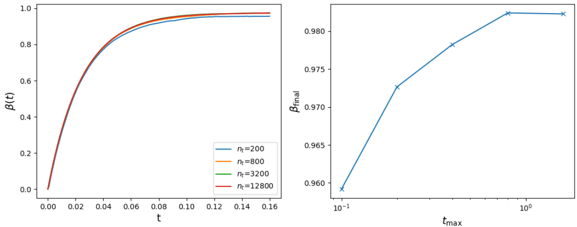
Figure 2: Convergence of \beta(t) at the representative point (g/\gamma, \kappa/\gamma) = (10^4, 10^7) . Left: \beta(t) for several values of n_t . Right: final value \beta(t_{\text{max}}) as a function of t_{\text{max}} .
