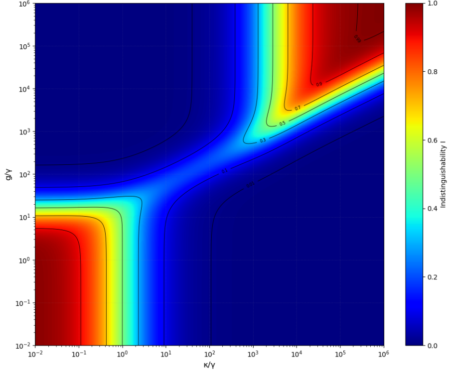
Figure 9: Indistinguishability I as a function of the coupling g and cavity decay rate \kappa , for \gamma^*/\gamma = 10^4 .
