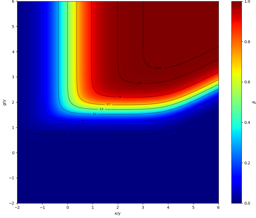
Figure 3: Efficiency \beta as a function of the coupling g and cavity decay rate \kappa , for a fixed ratio \gamma^*/\gamma = 10^4 .
