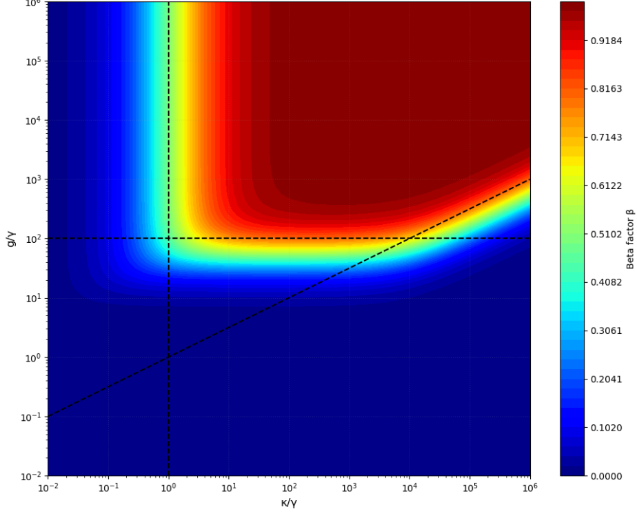
Figure 10: The high-beta region, delimited by the slope 1/2 line, the horizontal line at g/\gamma = \sqrt{\gamma^*/\gamma} and the vertical line at \kappa/\gamma = 1 for \gamma^*/\gamma = 10^4
