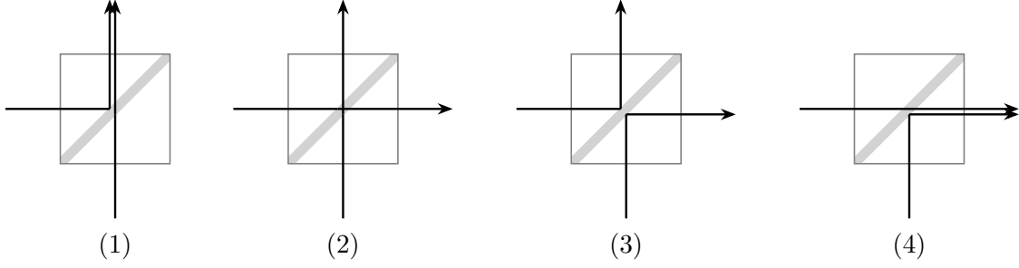
Figure 6: The four scattering amplitudes contributing to the two-photon output.
