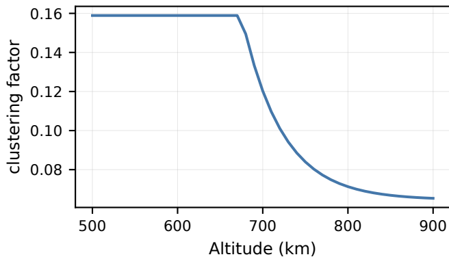
Calibrated clustering
