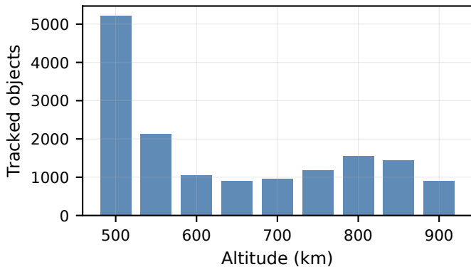
Calibrated clustering
