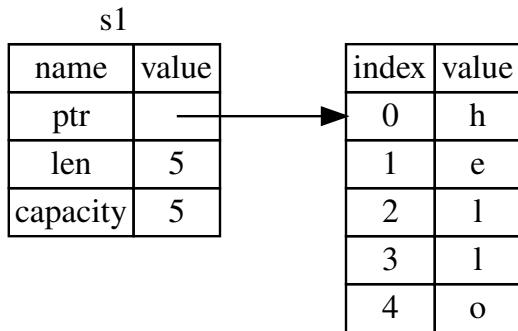
Figure 4-1: The representation in memory of a String holding the value "hello" bound to s1
