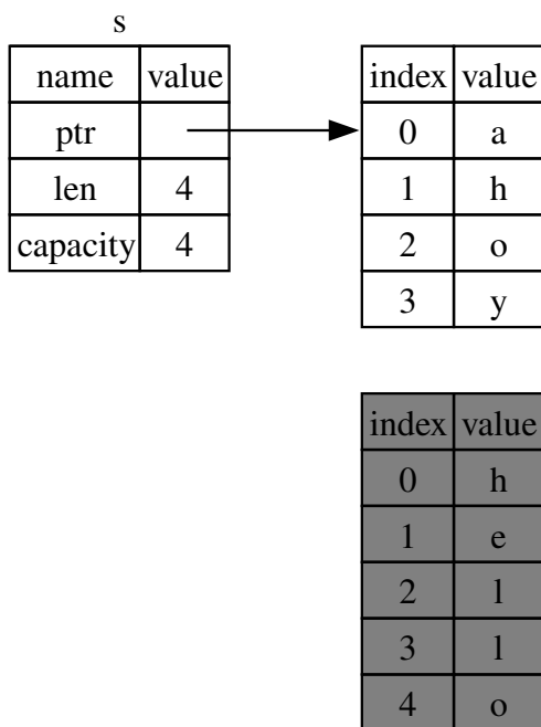
Figure 4-5: The representation in memory after the initial value has been replaced in its entirety
