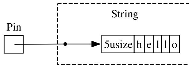
Figure 17.8: Figure 17-8: Pinning a ‘String’; the dotted line indicates that the ‘String’ implements the ‘Unpin’ trait and thus is not pinned
