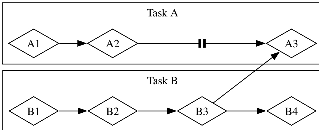
Figure 17.3: Figure 17-3: A partially parallel workflow, where work happens on Task A and Task B independently until Task A3 is blocked on the results of Task B3.
