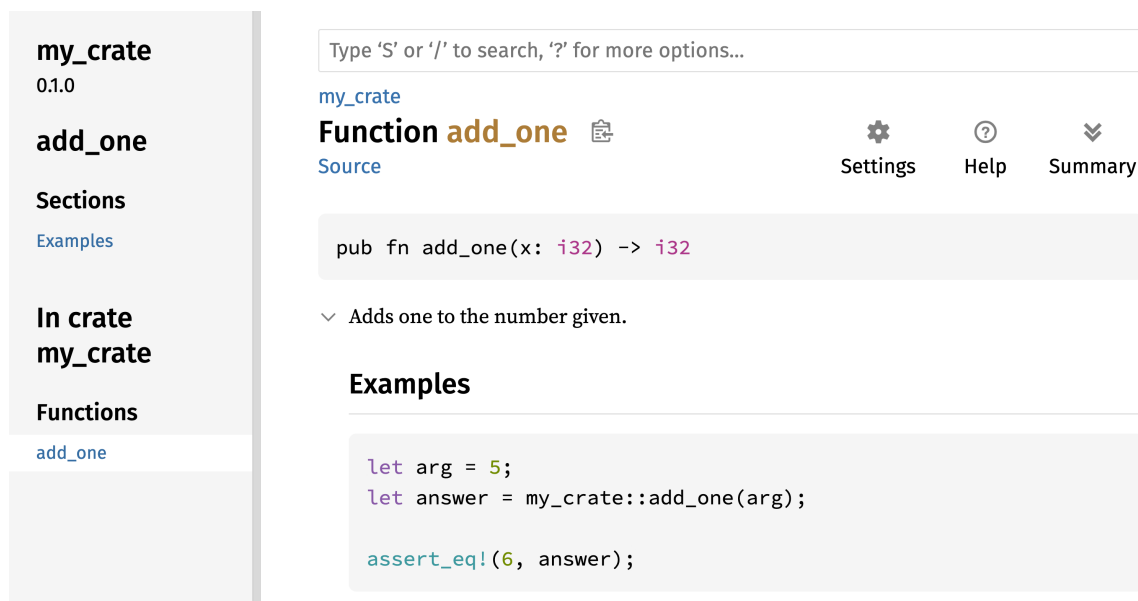
Figure 14-1: The HTML documentation for the add_one function
