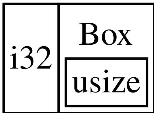
Figure 15-2: A List that is not infinitely sized, because Cons holds a Box
