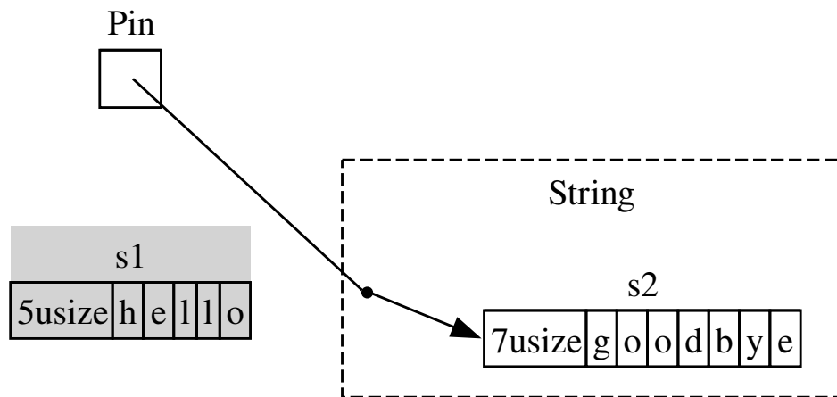
Figure 17.9: Figure 17-9: Replacing the ‘String’ with an entirely different ‘String’ in memory
