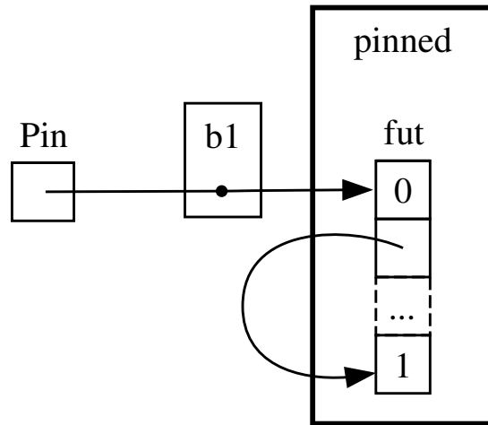
Figure 17.6: Figure 17-6: Pinning a 'Box' that points to a self-referential future type
