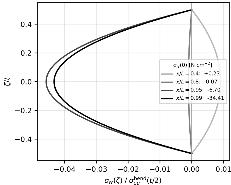
(b) \sigma_{rr} : quadratic, zero at both faces
