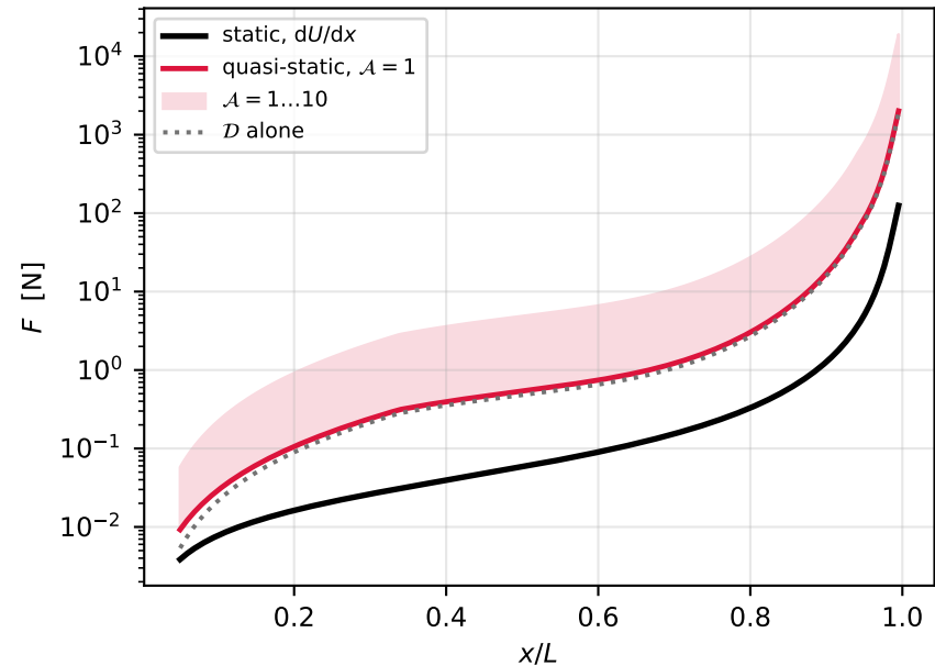
(a) static vs quasi-static force
