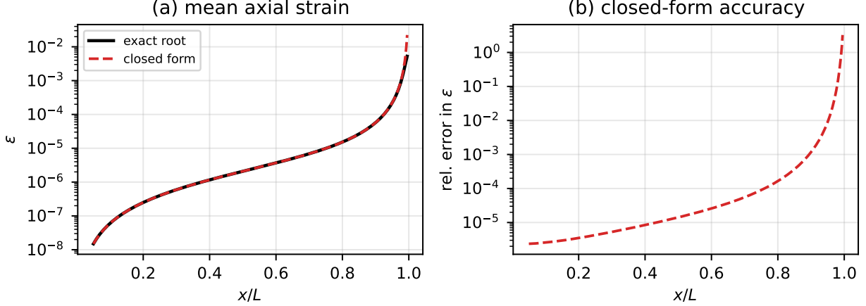
Figure 2: (a) The mean axial strain, on a logarithmic scale: the closed form Eq. (97) against the exact root of Eq. (91). The two are indistinguishable over almost the whole range. The strain is tiny but strictly positive everywhere, and rises steeply only in the last few percent of extension. (b) Relative error of the closed form: below 10^{-3} out to x/L \approx 0.89 and below 1% out to x/L \approx 0.95 , rising sharply thereafter as the extension approaches the crossover of Eq. (102), where the expansion’s own validity condition fails.
