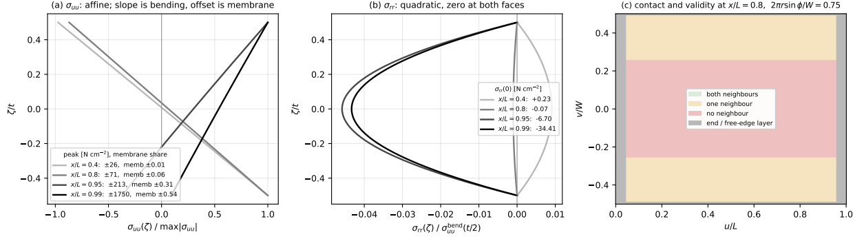
Figure 6: Fields of the minimizing state, and where they are valid. (a) \sigma_{uu} is affine in \zeta by Eq. (118): the offset is membrane, the slope bending, and the legend gives the peak value and the membrane share of it. The slope changes sign between x/L = 0.8 and 0.95 . (b) \sigma_{rr} is the quadratic bump of Eq. (133), normalized by the bending stress at the surface; it vanishes at both faces and changes sign near x/L \approx 0.7 . (c) The (u, v) plane at x/L = 0.8 : the boundary layers assumption 10 discards, and the contact gates of Eqs. (54)–(55). Inside the valid region the stress field is uniform in (u, v) by construction, which is why no stress is plotted over it.
