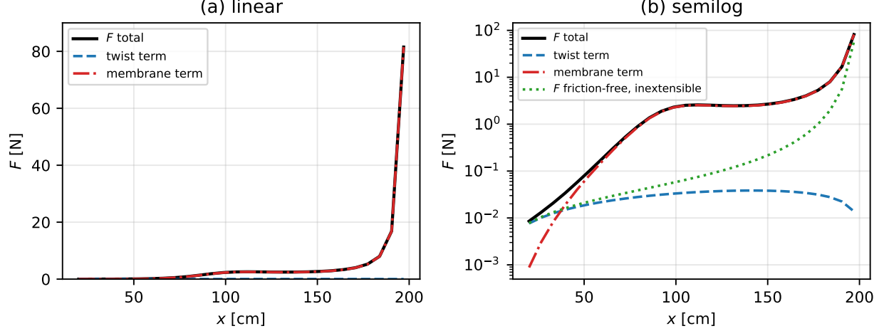
Figure 9: Force–displacement, linear and semilogarithmic, showing the two additive terms of Eq. (167). The twist term is friction-independent and dominates below x/L \approx 0.2 ; the capstan-amplified membrane term dominates above it. The dotted curve is the friction-free closed form Eq. (111) for comparison, which the total exceeds once the gain \mathcal{A} of Eq. (166) departs from unity. The total spans 0.0085 to 82 N with a logarithmic slope that increases with x , i.e. growth faster than any single exponential.
