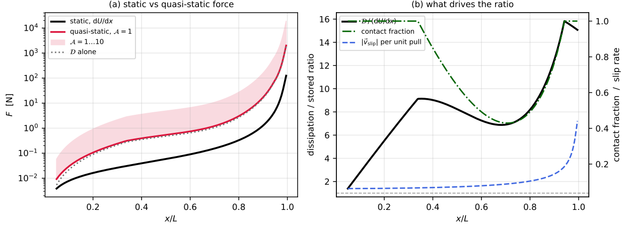
Figure 7: (a) The static force of Eq. (90) against the quasi-static force of Eq. (152), with the band showing capstan gains \mathcal{A} = 1 to 10. (b) The ratio, and the two factors that drive it: the contact fraction from the gates (54)–(55) and the slip rate (153). The kink near x/L \approx 0.35 is the gate closing, the recovery near 0.95 is it reopening.
