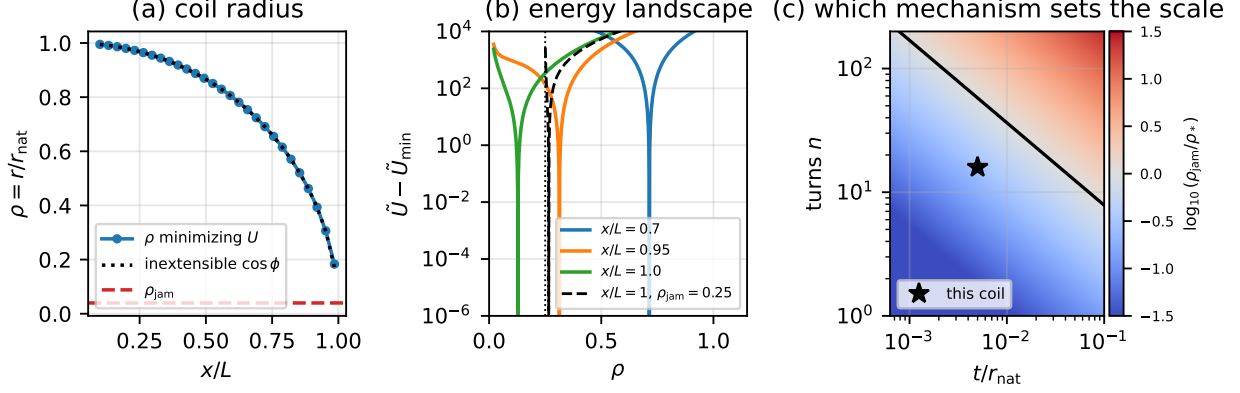
Figure 3: (a) The energy-minimizing radius from Eq. (91), against the inextensible \cos \phi and the packing floor Eq. (19). The minimizer tracks the inextensible value closely, consistent with \Gamma \gg 1 , and decreases monotonically throughout — there is no turning point. (b) The energy landscape of Eq. (106) at three extensions with \rho_{\text{jam}} = 0 , plus one case with \rho_{\text{jam}} = 0.25 (dashed) showing the packing divergence appear as an asymptote of the same energy. The well is single and deep, so the minimization is unambiguous. (c) Which mechanism sets the radius scale, from Eq. (107): the black contour is \rho_{\text{jam}} = \rho_* , and the star marks the coil of Section 9.13.
