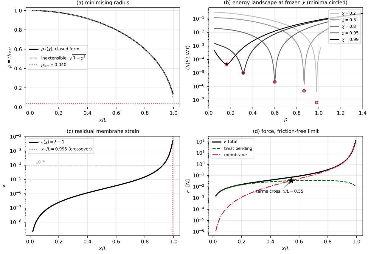
Figure 5: The closed-form solution of Eq. (87) for the coil of Section 9.13. (a) The minimizing radius, against the inextensible \sqrt{1-\chi^2} and the packing scale \rho_{\text{jam}} . (b) The energy at five frozen extensions, showing one interior minimum apiece; the minima are circled. (c) The residual membrane strain, with the crossover x_*/L of Eq. (102) marked. (d) The force and its two terms from Eq. (90), in the friction-free limit \mathcal{A} = 1 .
