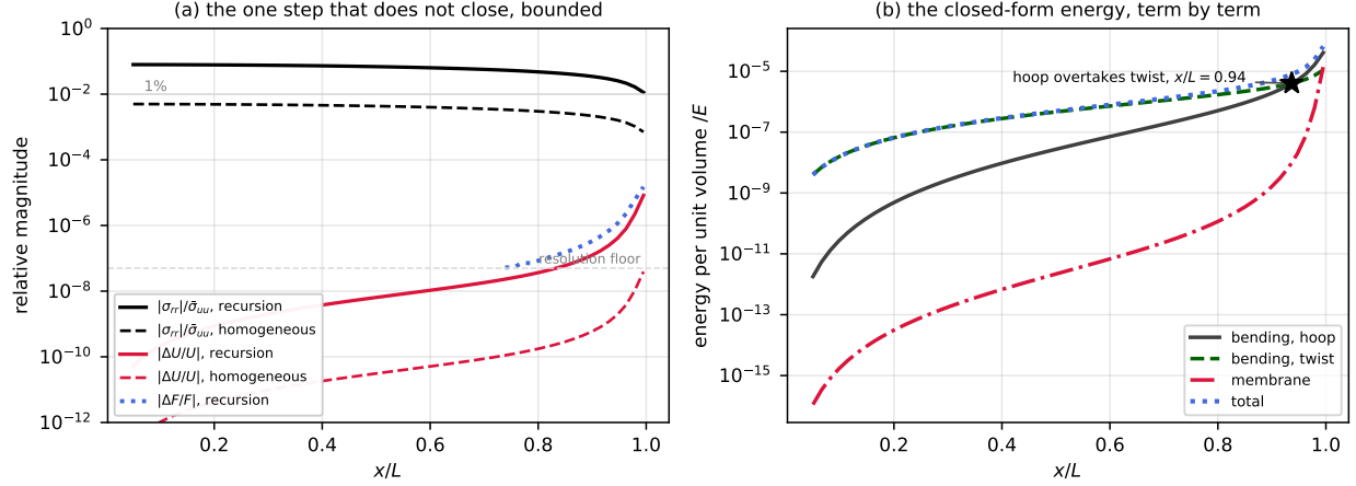
Figure 4: (a) The flagged step of Section 7.4, bounded. The transverse pressure is shown for the two closures — the single-layer jump that assumption 10 permits, and the full accumulation imported from the recursion — together with the change each makes to the energy and to F . The largest effect anywhere is 8 \times 10^{-6} in the energy and 1.5 \times 10^{-5} in the force, so the unresolved boundary value does not reach the deliverable. |\Delta F/F| is drawn only above the sweep’s finite-difference floor. (b) The three terms of Eq. (87) evaluated along the minimizing path \rho(\chi) . Twist bending carries the energy for most of the pull, the hoop term overtakes it near x/L = 0.94 , and the membrane term — negligible over four decades — climbs steeply enough at the end to reach a quarter of the bending energy by x/L = 0.995 .
