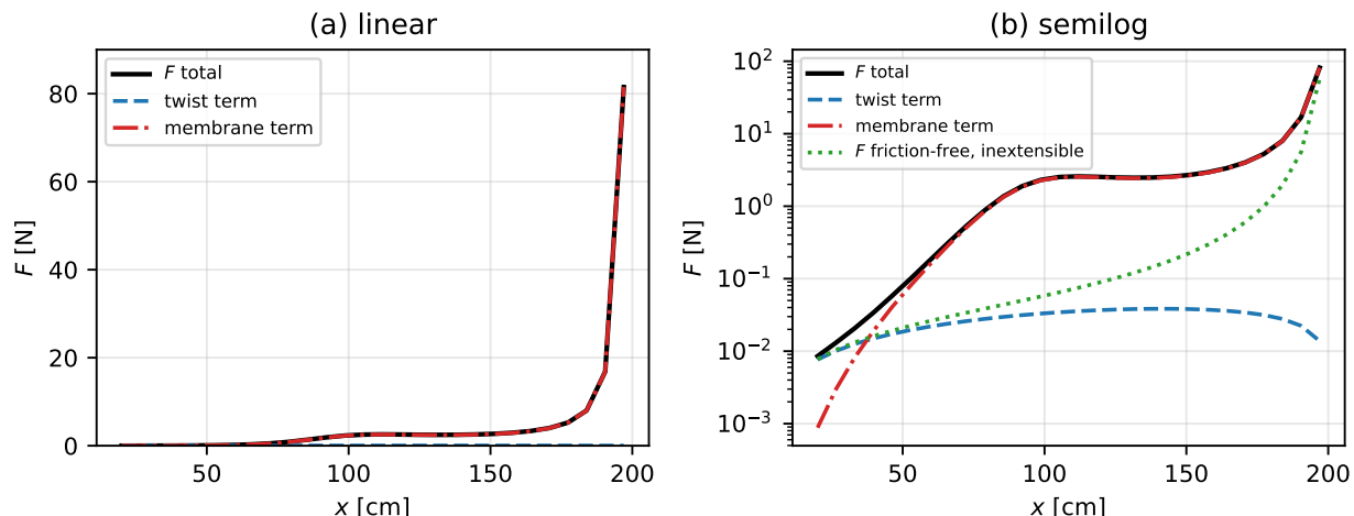
Figure 5: Force–displacement, linear and semilogarithmic, showing the two additive terms of Eq. (97). The twist term is friction-independent and dominates below x/L \approx 0.2 ; the capstan-amplified membrane term dominates above it. The dotted curve is the friction-free closed form Eq. (87) for comparison, which the total exceeds once the gain \mathcal{A} of Eq. (96) departs from unity. The total spans 0.0085 to 82 N with a logarithmic slope that increases with x , i.e. growth faster than any single exponential.
