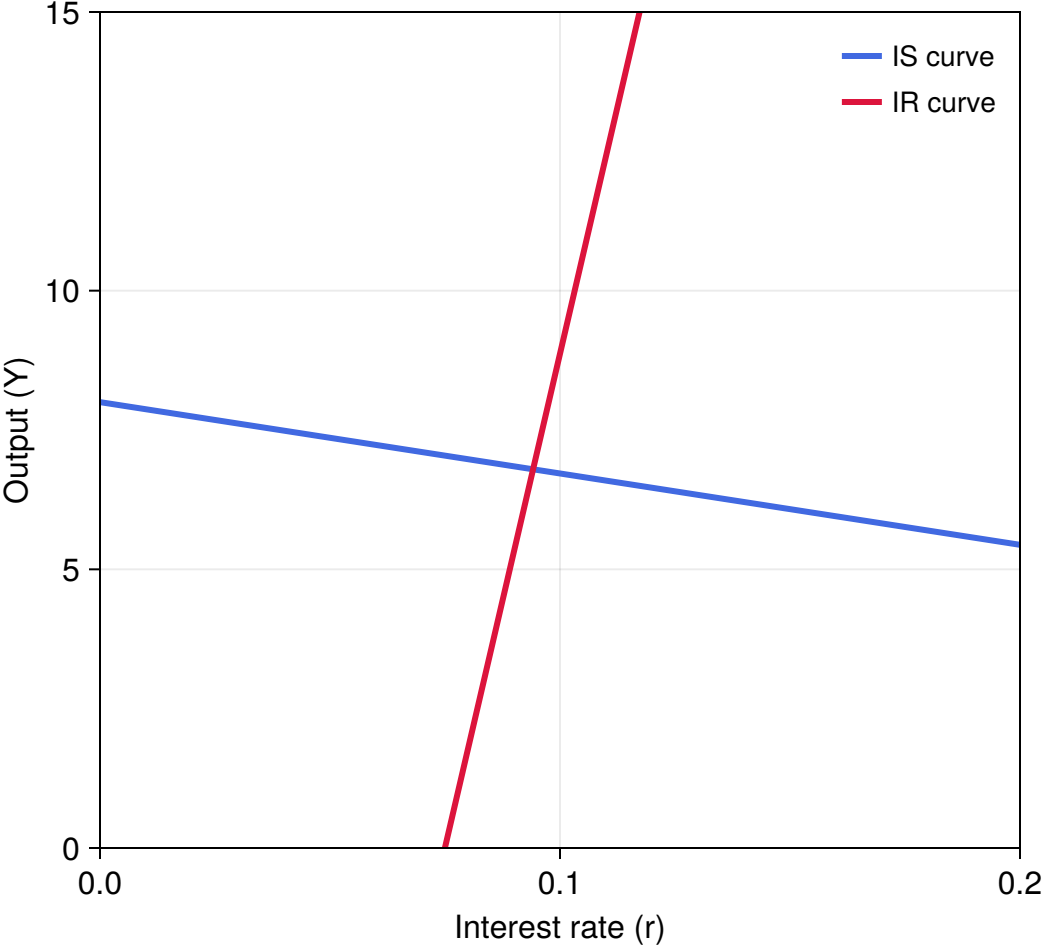
Goods market and interest-rate rule
