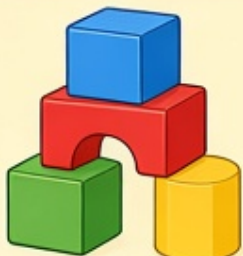
blocks
