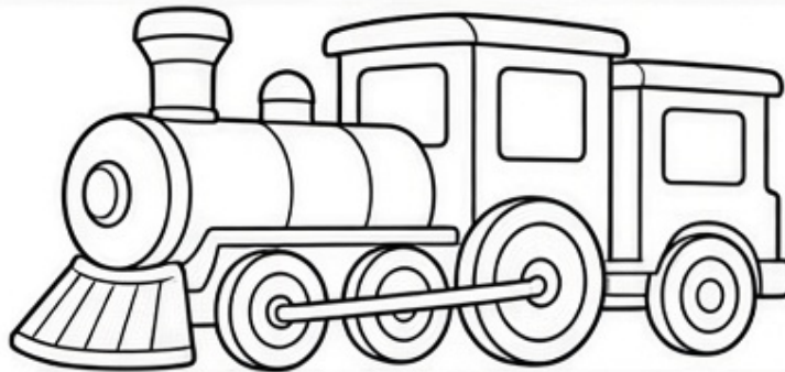
train
