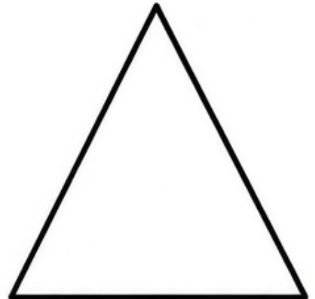
triangle
