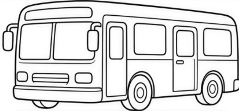
bus
