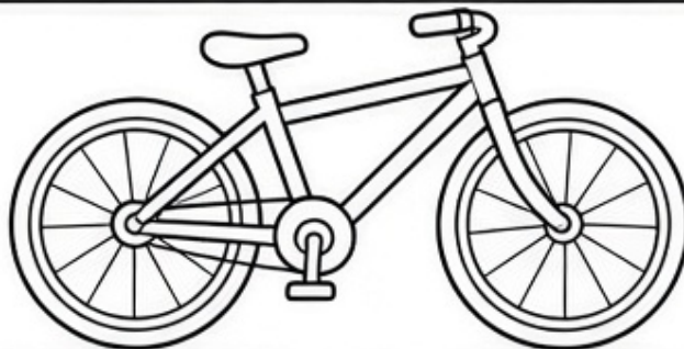
bike
