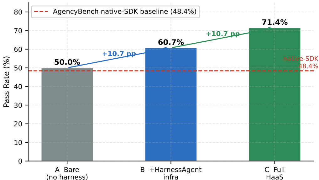
Figure 1 — AgencyBench-V2 Harness Ablation 28 tasks · 6 capability dimensions · seed=42
