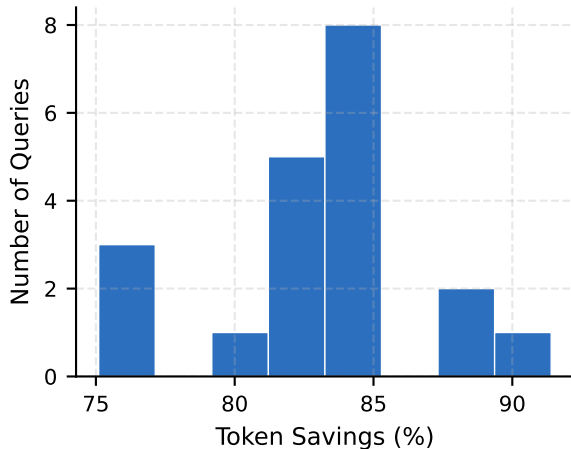
Savings Distribution (n=20 queries)
