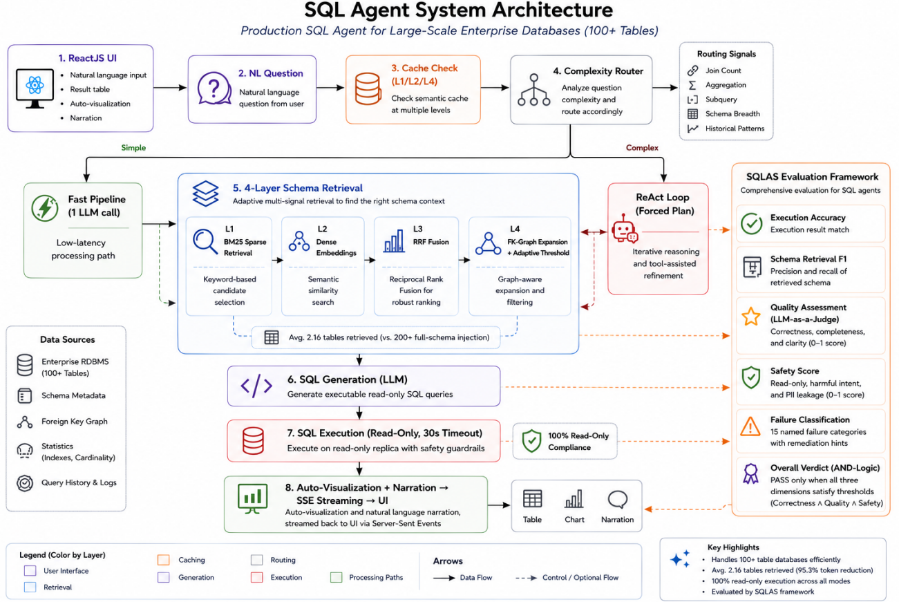
Fig. 1. NexusSQL system architecture. The 4-layer adaptive retrieval pipeline (L1: BM25 Sparse → L2: Dense Embeddings → L3: RRF Fusion → L4: FK-Graph + Adaptive Threshold) selects an average of 2.16 tables from 100+ table schemas, reducing prompt tokens by 95.3% versus full-schema injection. Simple queries take the Fast Pipeline (1 LLM call); complex queries use the ReAct Agent with a mandatory forced-plan step. SQLAS provides end-to-end evaluation across correctness, quality, and safety dimensions with AND-logic verdict.
