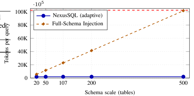
Fig. 3. Token cost per query vs schema scale. NexusSQL’s adaptive retrieval stays constant at ≈1,932 tokens regardless of schema size. Full-schema injection grows linearly, exceeding the 128K context window limit beyond ≈640 tables and failing entirely.
