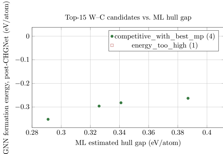
Figure 3.1: Scatter of post-CHGNet GNN formation energy vs. ML-estimated hull gap. Pareto-front candidates are in the lower-left.
