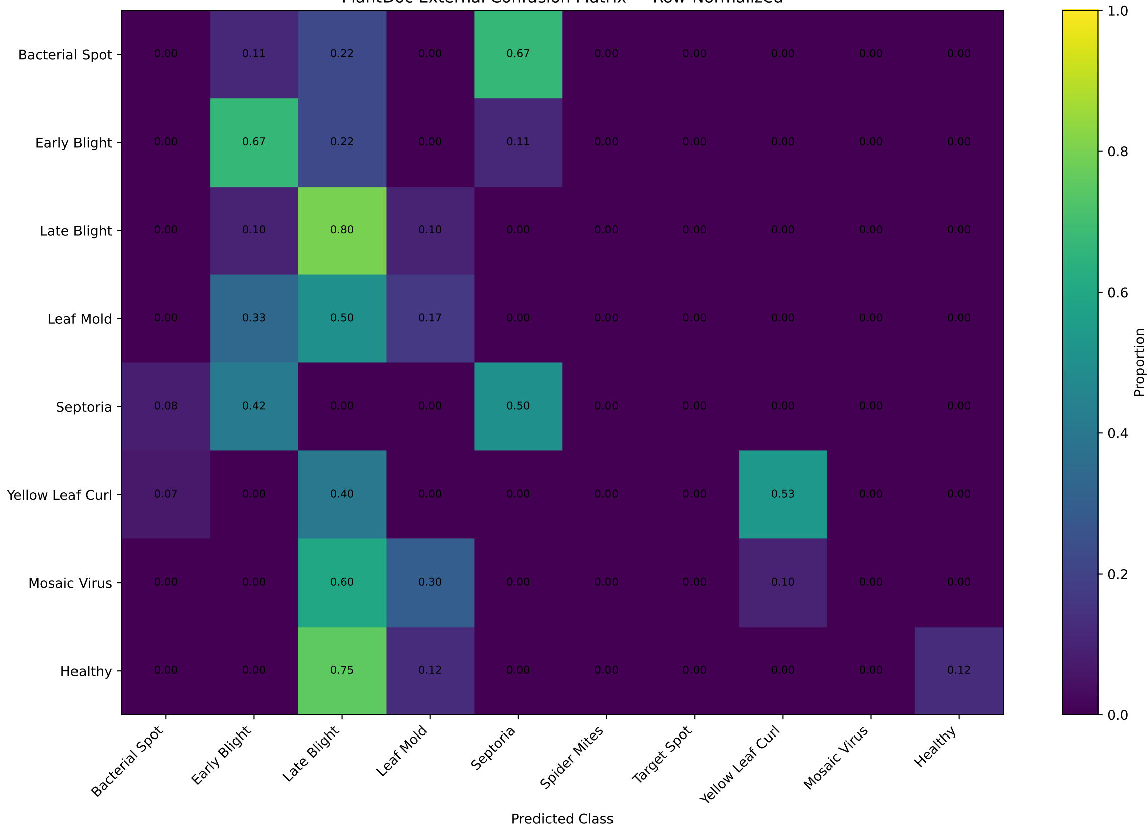
PlantDoc External Confusion Matrix — Row-Normalized
