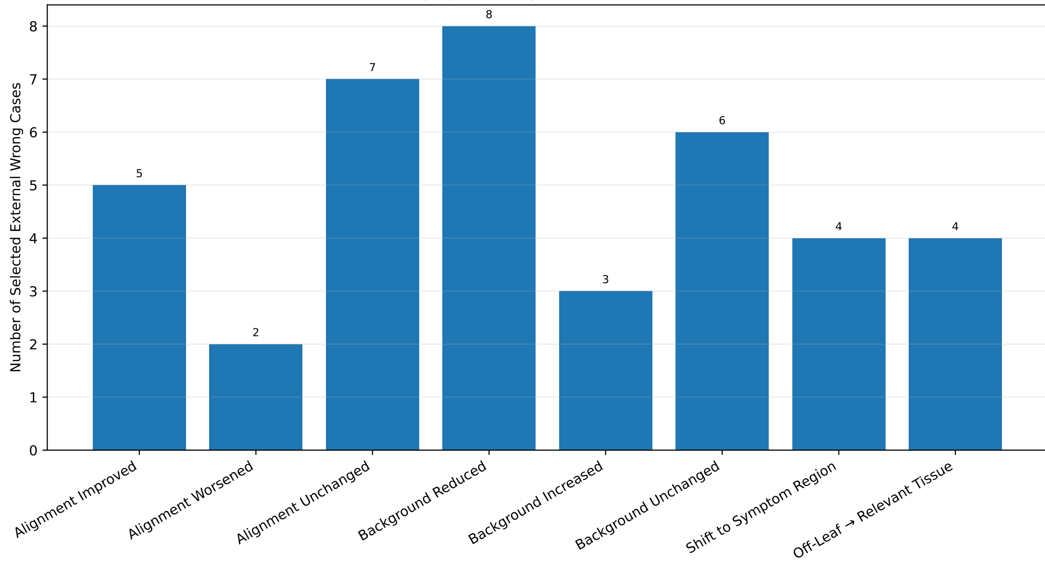
Effect of Changing CAM Target from Predicted to True Class
