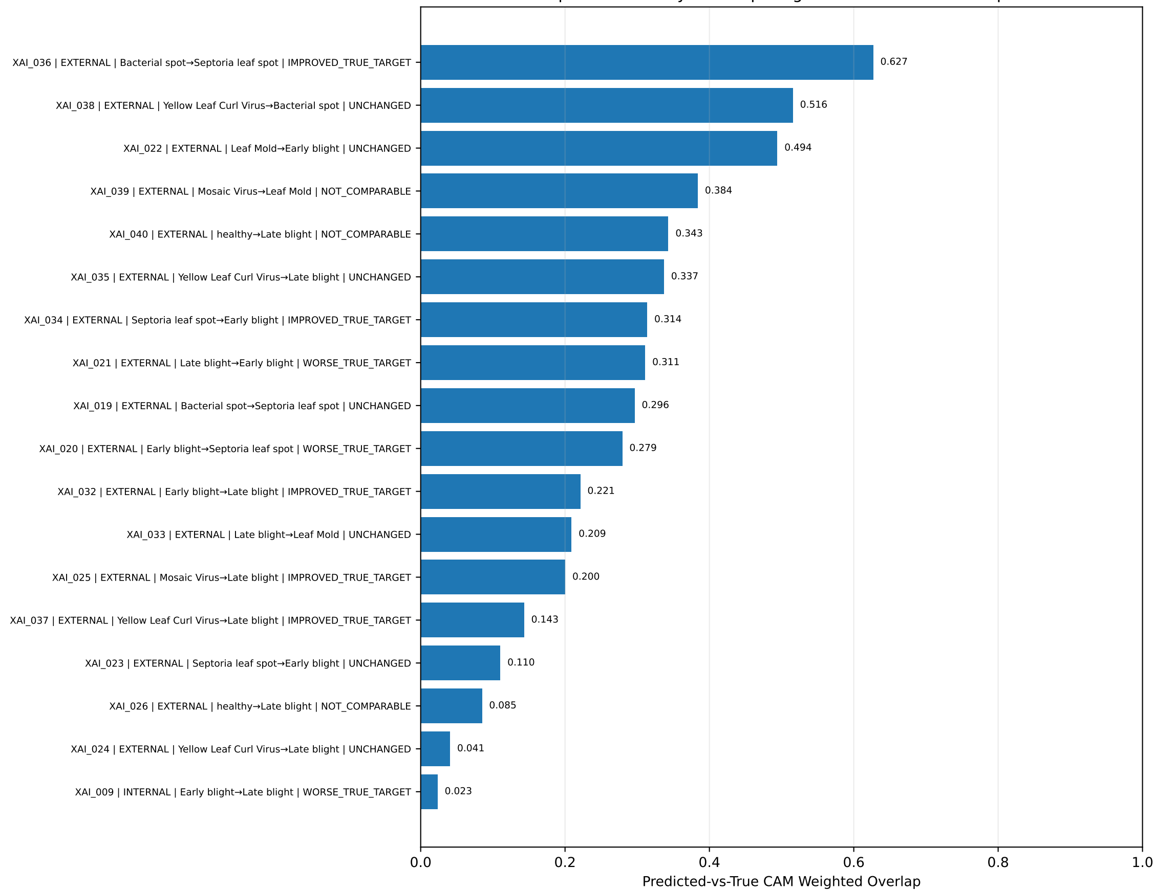
Spatial Similarity of Competing-Class Grad-CAM++ Maps
