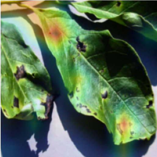
True-class CAM
