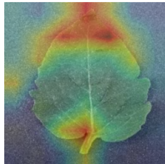
Predicted-class Grad-CAM++
