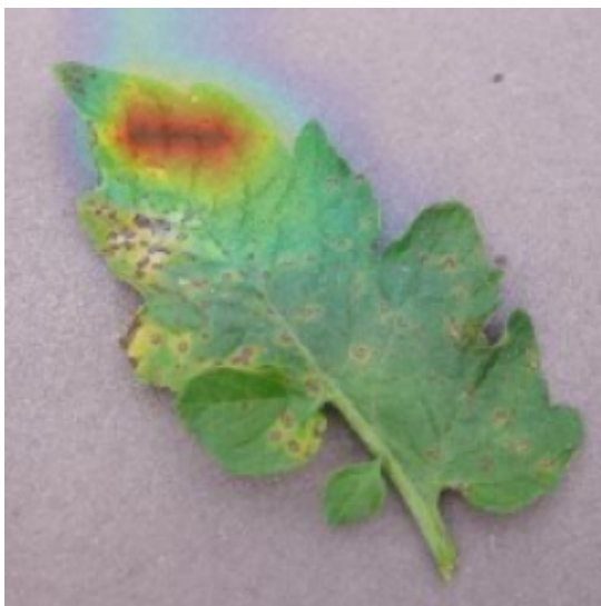
Predicted-class Grad-CAM++
