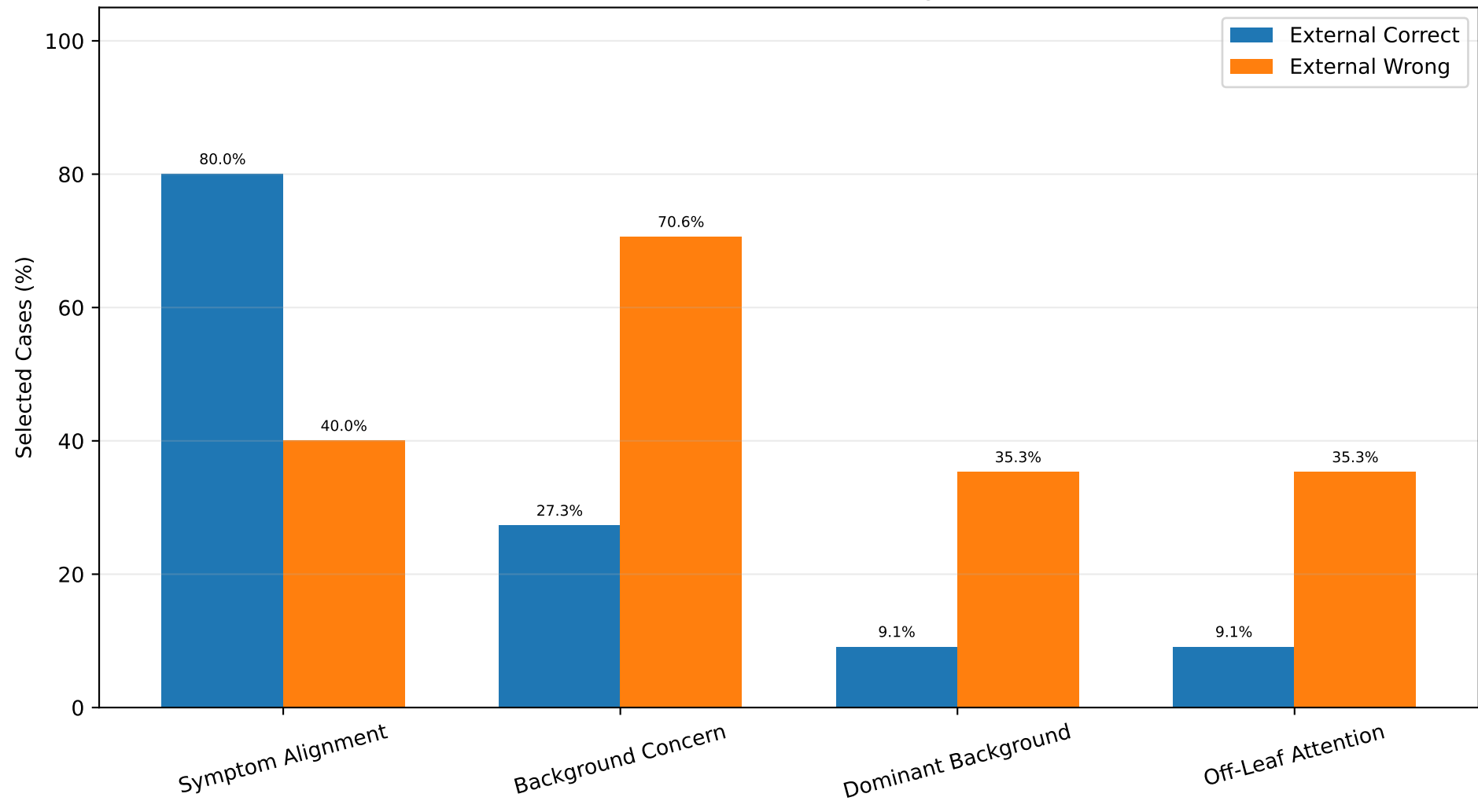
External PlantDoc: Correct vs Wrong XAI Patterns
