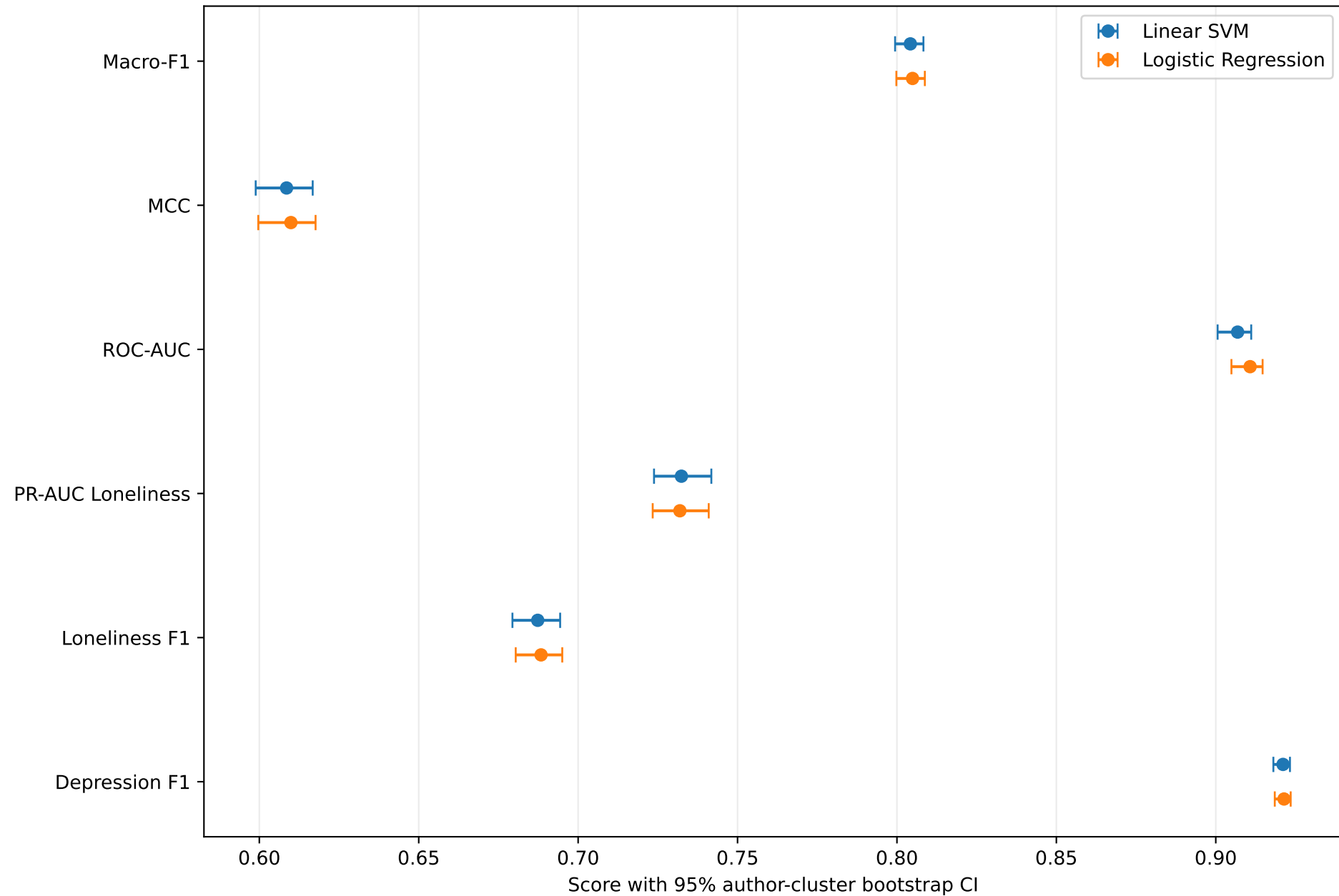
Independent Test Performance Uncertainty
