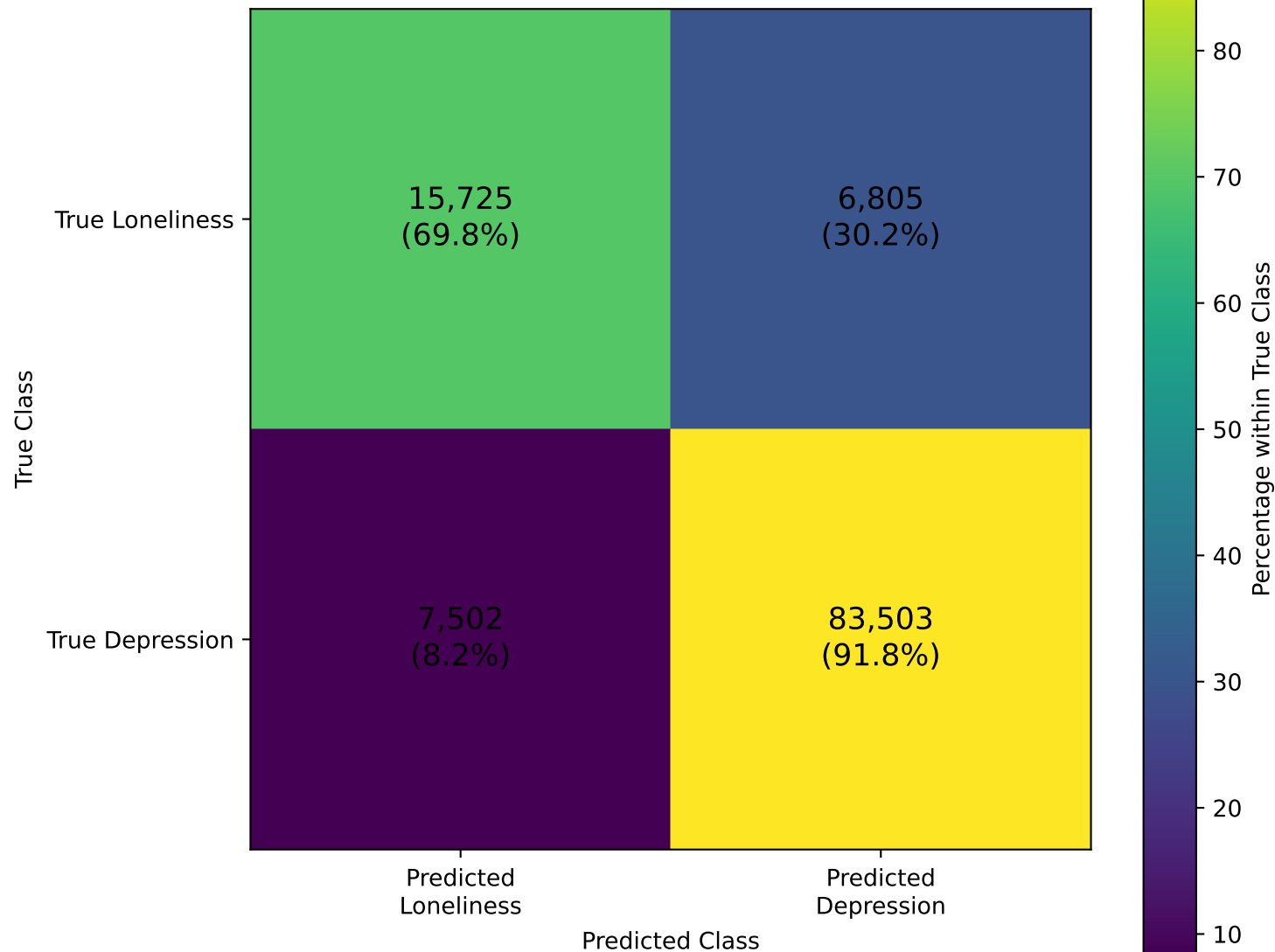
Final Test Confusion Matrix — Linear SVM
