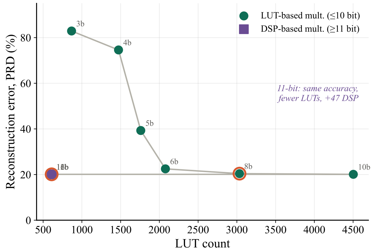
Accuracy vs. LUT cost (Pareto front)
