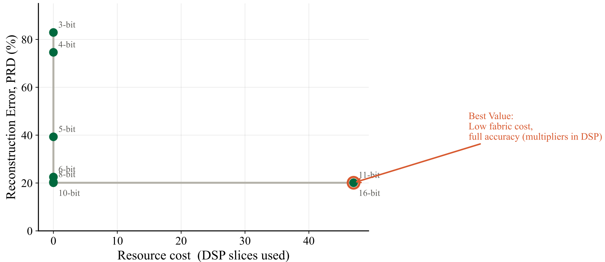
Accuracy vs. Resource Cost
