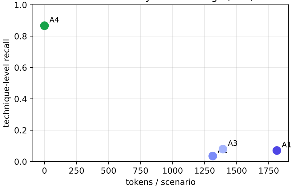
Cost vs accuracy — multi-stage (32B)
