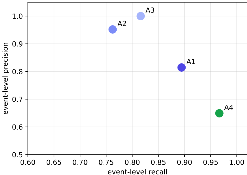
Event-level: LLM more precise than rules (multi-stage, 32B)
