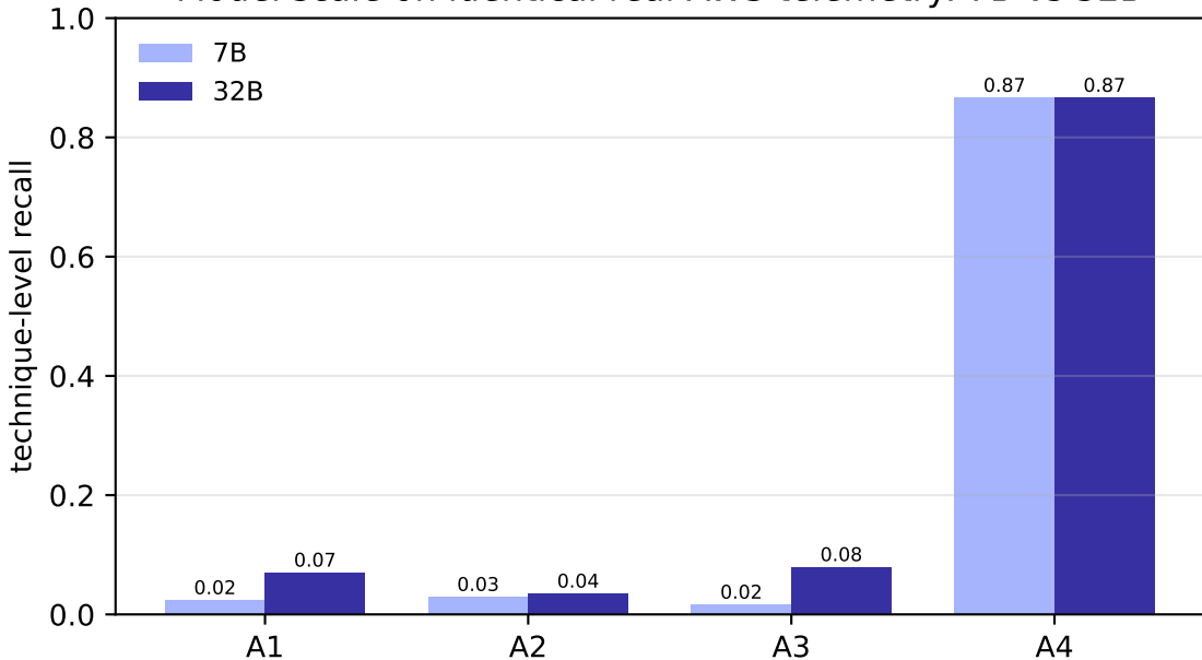
Model scale on identical real-AWS telemetry: 7B vs 32B
