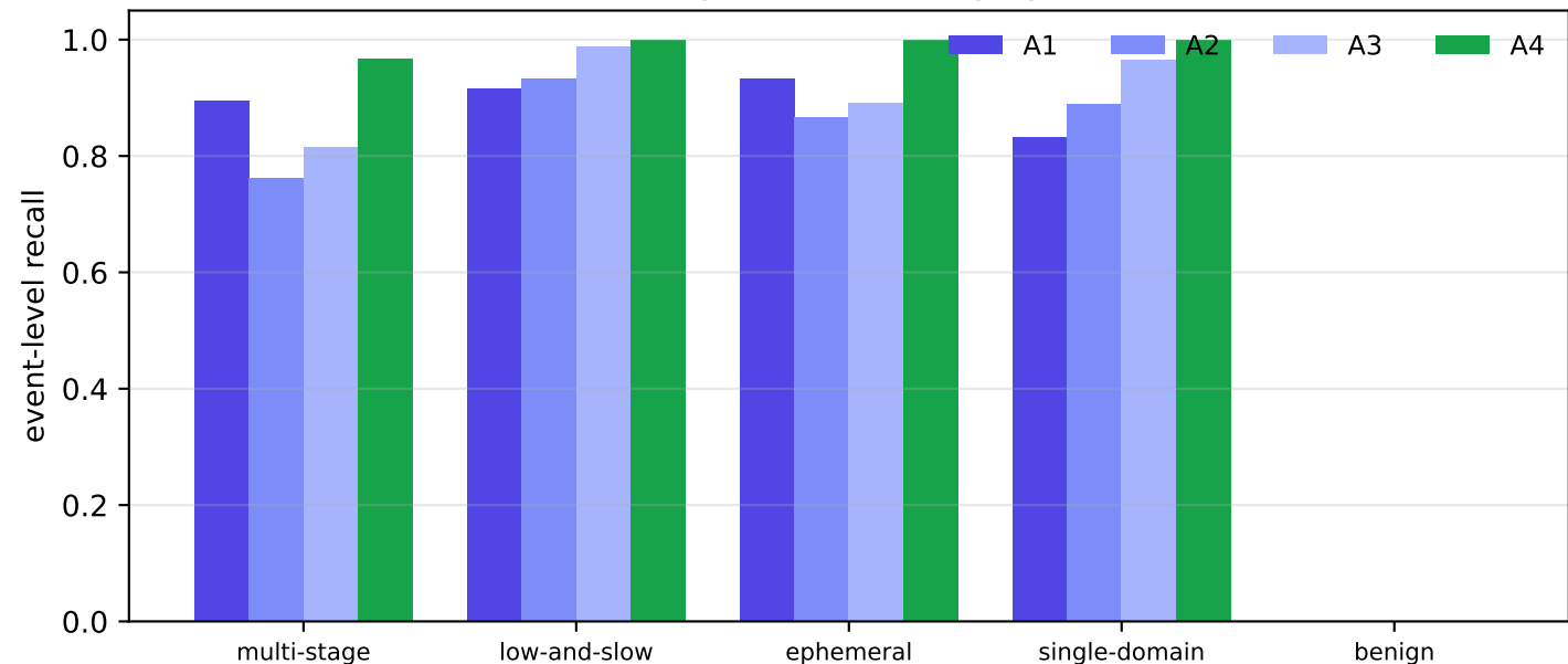
Event-level recall by arm and category (32B, real-AWS)
