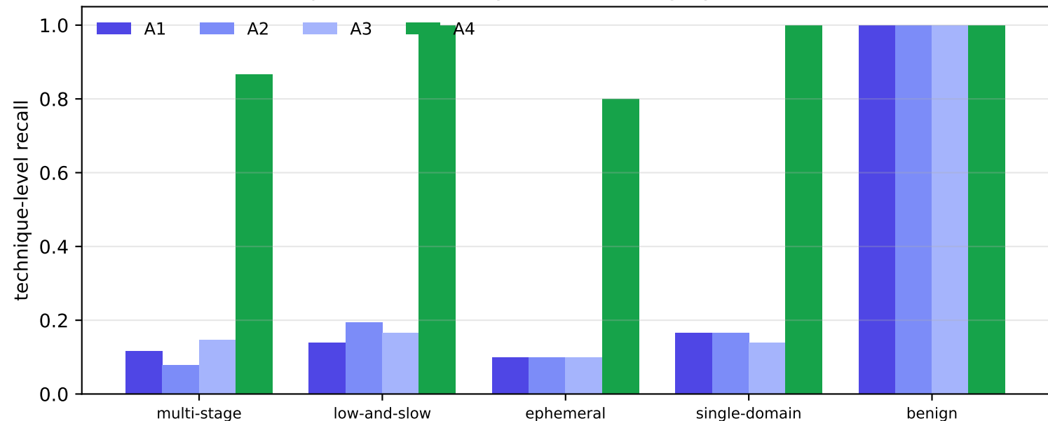
Technique-level recall by arm and category (32B, real-AWS)
